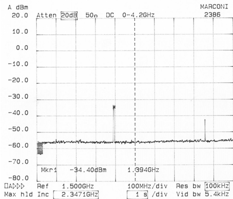
Spurious Emissions 1-2GHz
