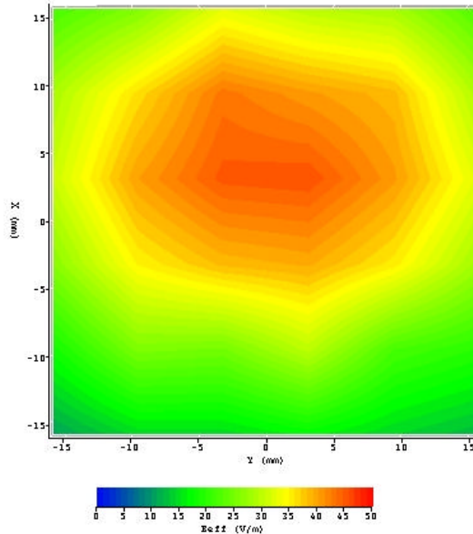
Validation Measurement – 2450 MHz in Head tissue
