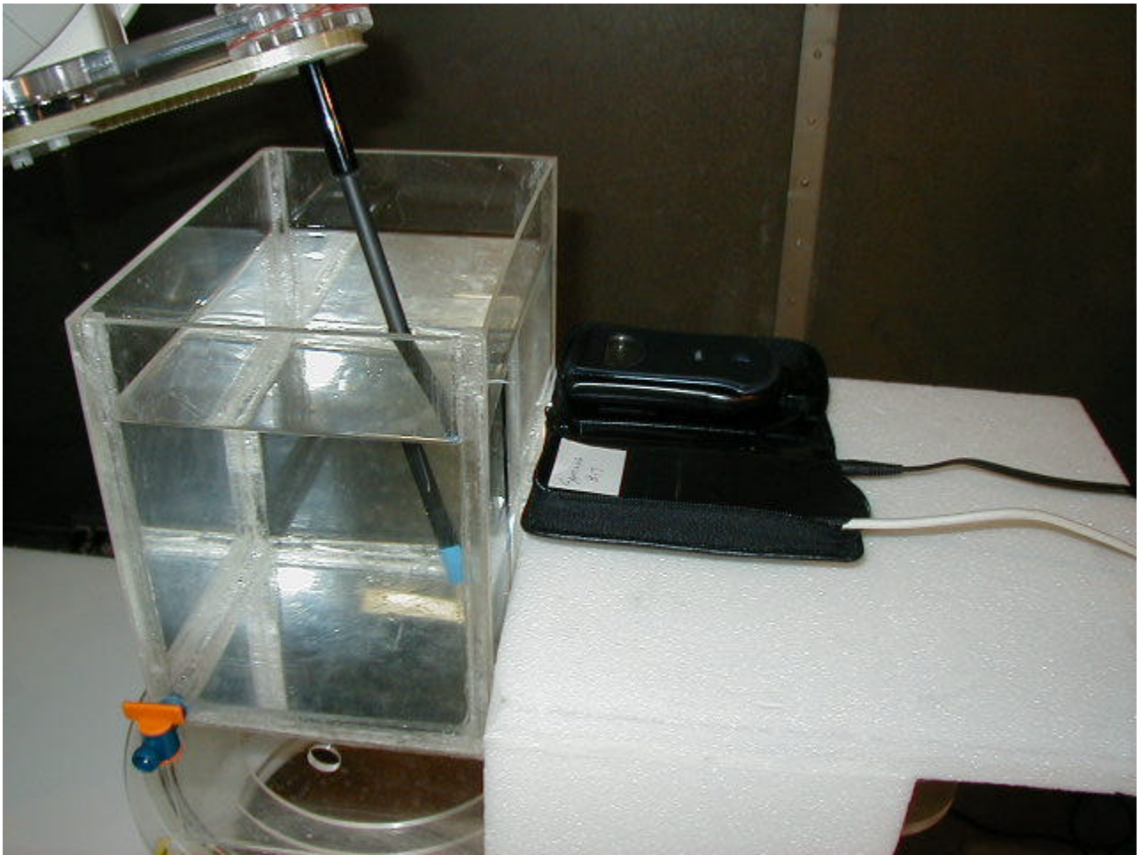
Figure S1. Setup Configuration 1
