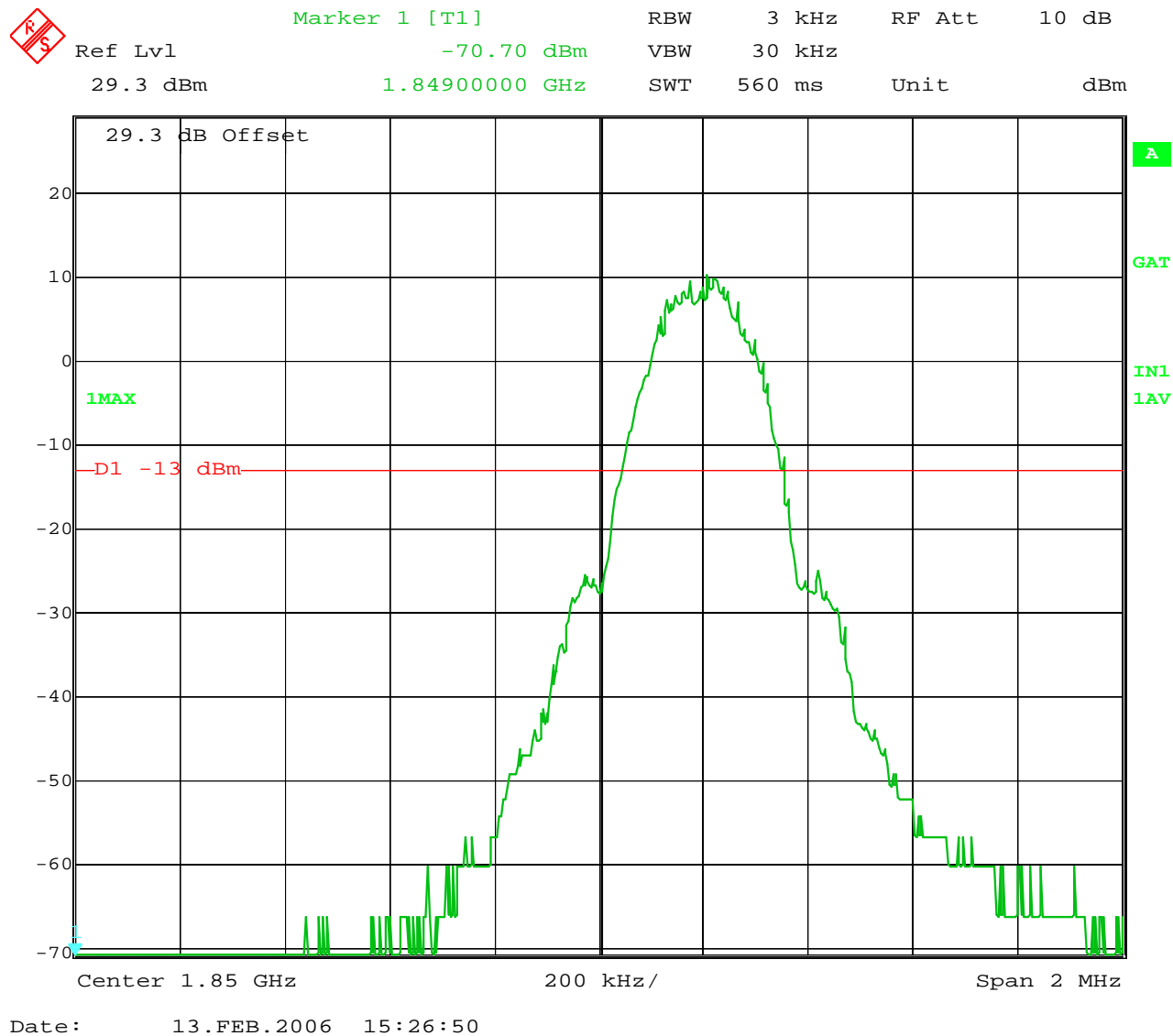
Figure 8-7: Emissions within 1 MHz of band edge, GSM 1900 Lower Band Edge
