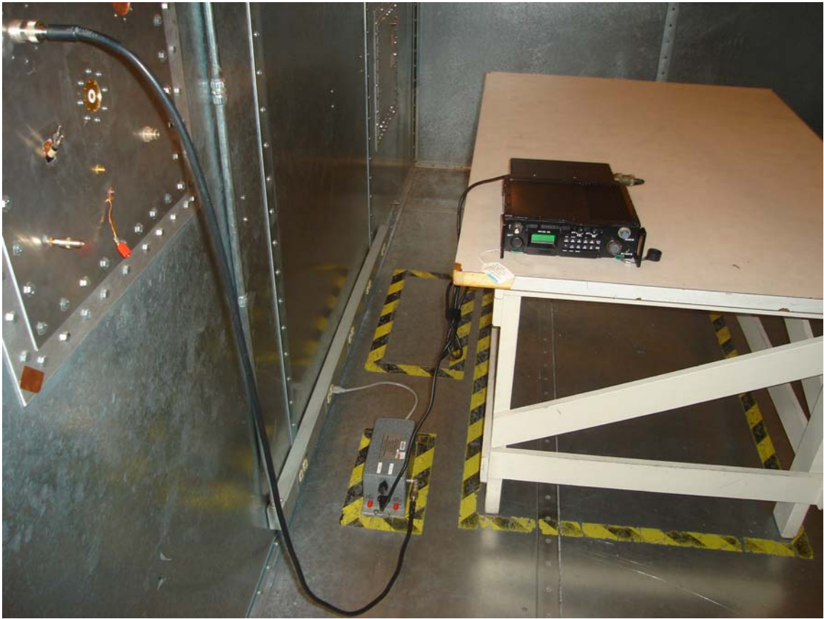
Figure 7.0-3 Powerline Conducted Emissions Test Setup
