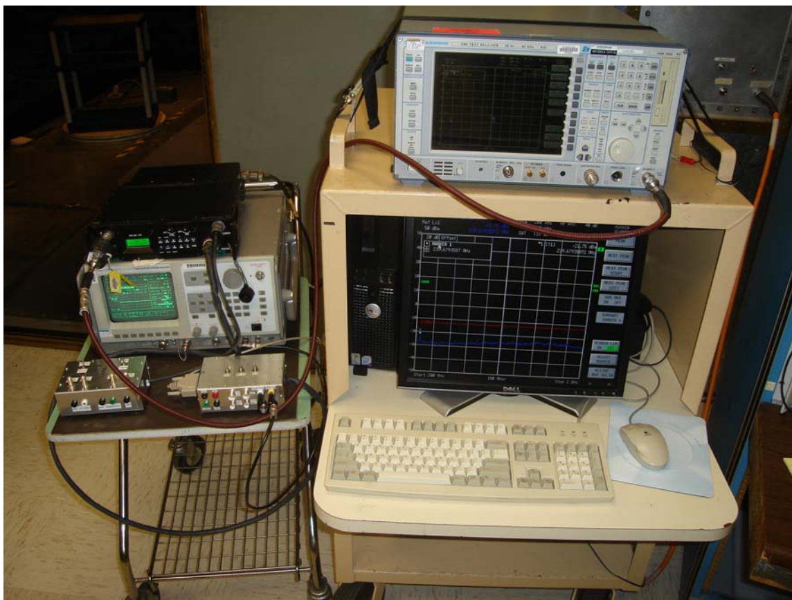
Figure 7.0-1 Antenna Port Conducted Emissions Test Setup
