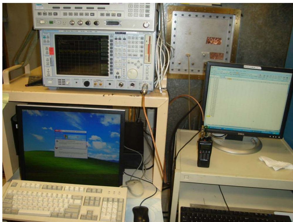
Figure 7.0-1 Front-End Conducted Emissions Test Setup
