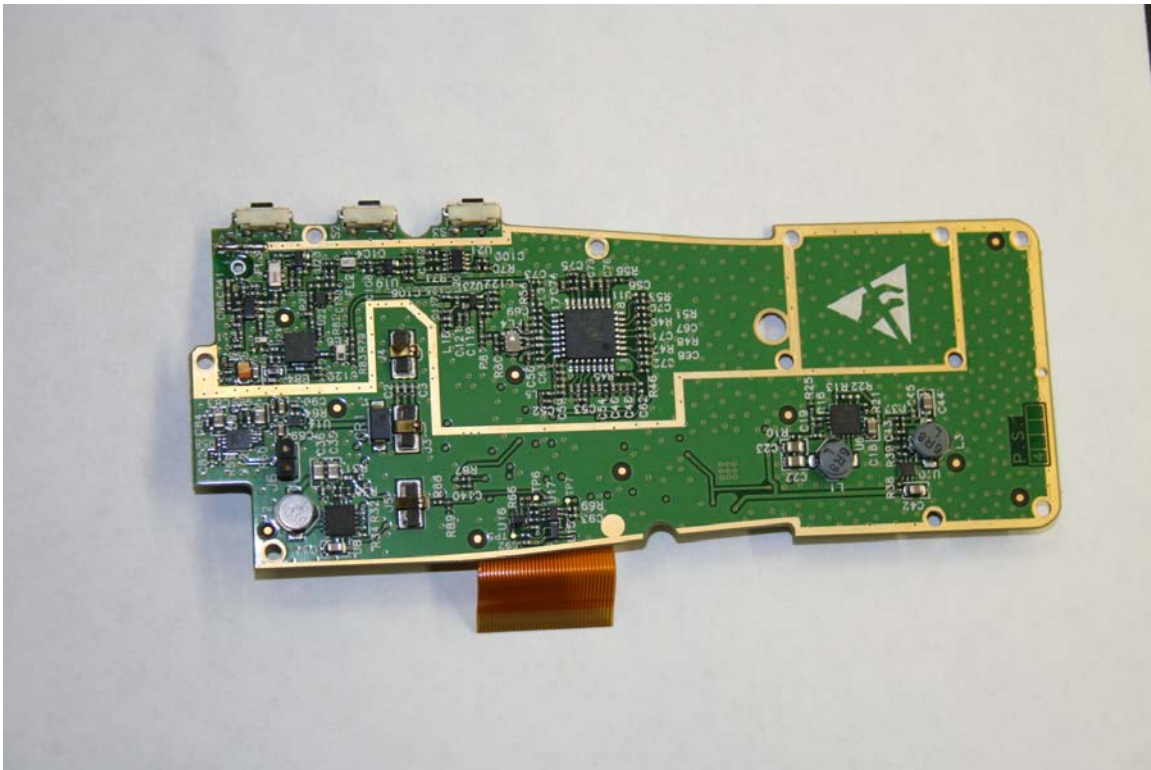
Figure 9.0-1 RF PCB (Top)
