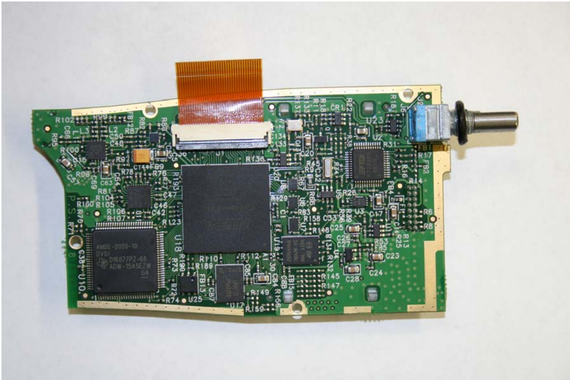
Figure 9.0-4 Control PCB (Bottom)
