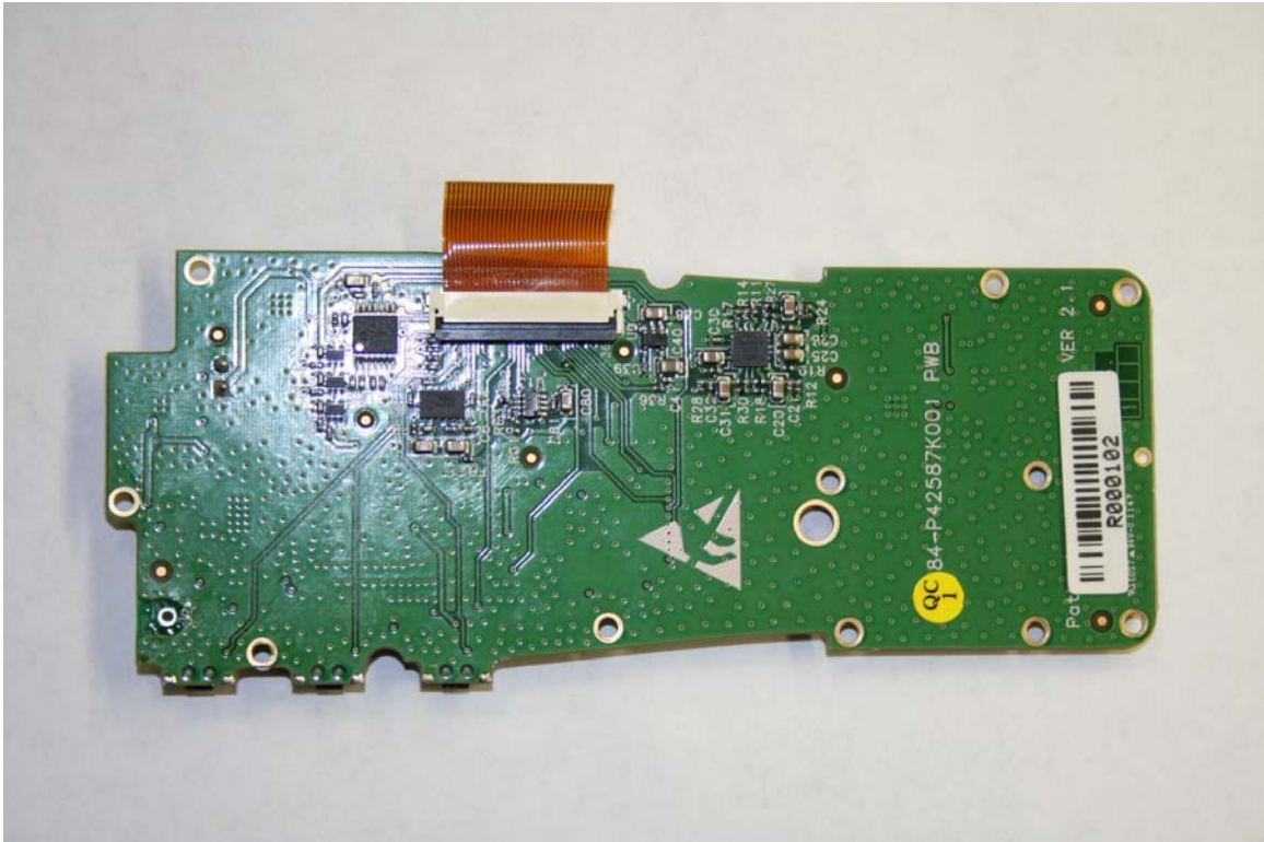
Figure 9.0-2 RF PCB (Bottom)
