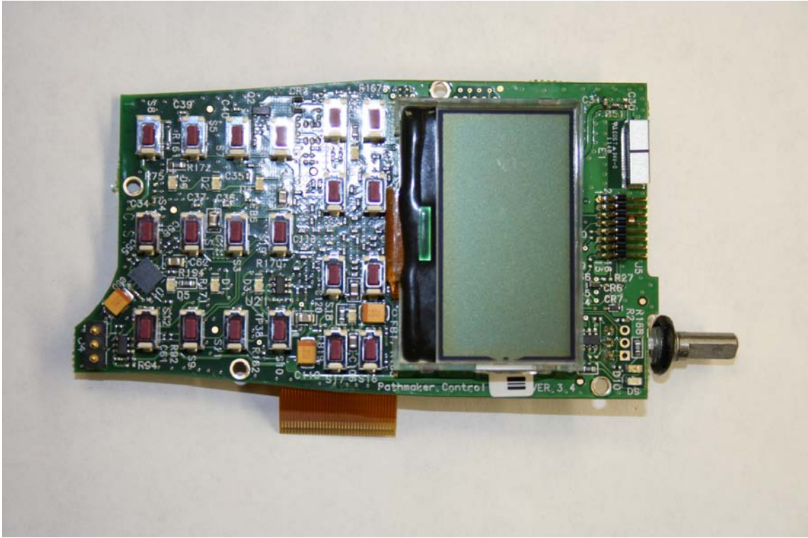
Figure 9.0-3 Control PCB (Top)
