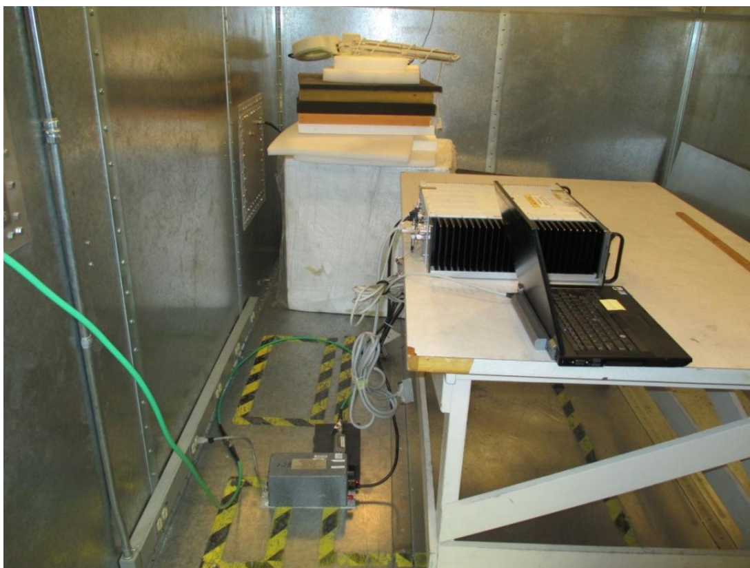
Figure 7.0-1 AC Conducted Emissions Test Setup
