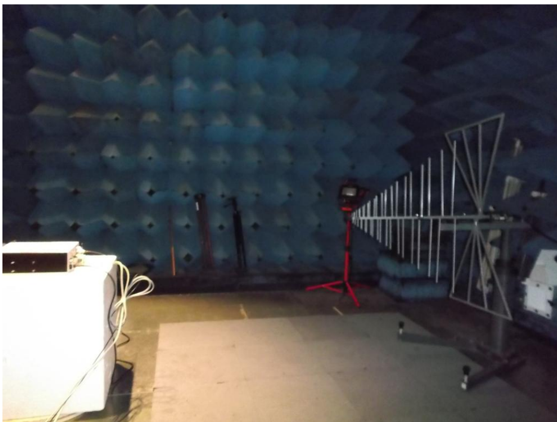
Figure 7.0-3 Radiated Emissions Test Setup (Pre-Scans/Anechoic Chamber)
