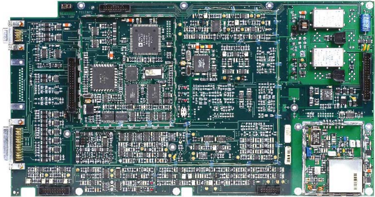
Figure 9.0-3 Control PCB Top without Shields
