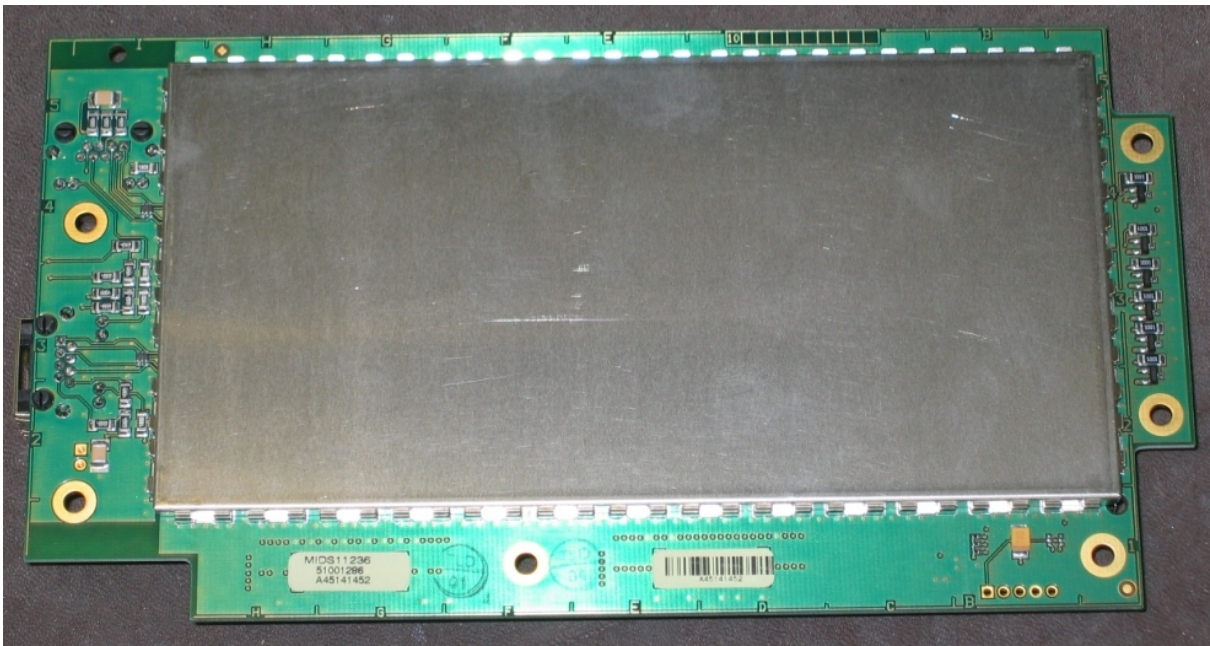
Figure 9.0-10 MIDS CCA Back with Shield
