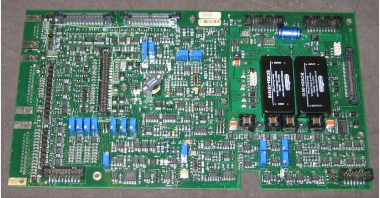
Figure 9.0-2 Control CCA Top
