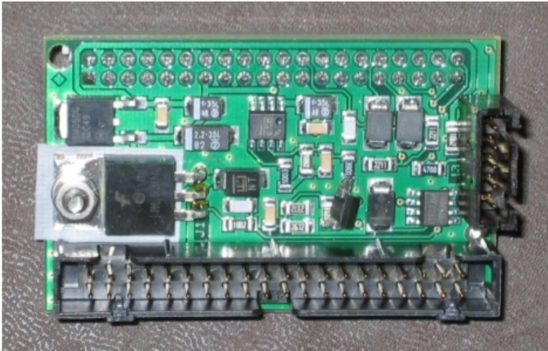
Figure 9.0-6 ADAP CCA Top
