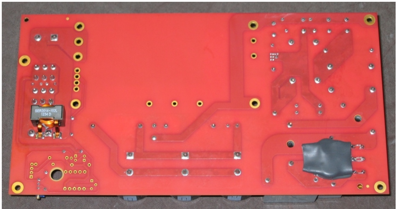
Figure 9.0-5 ALPF CCA Back
