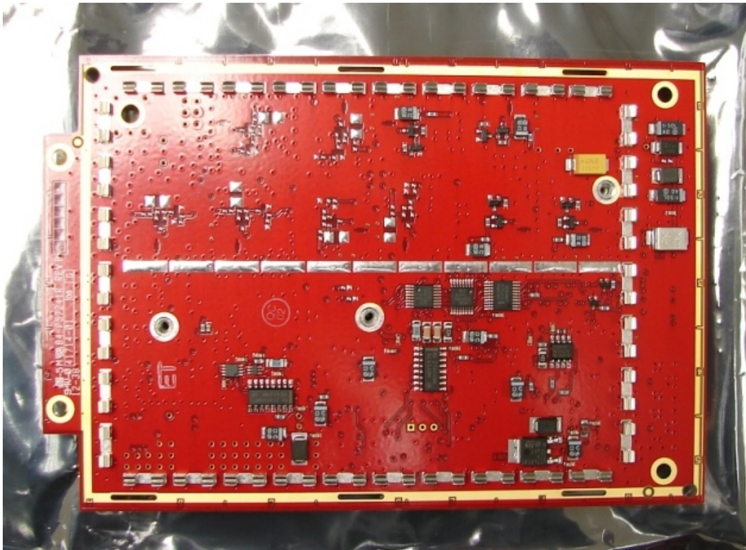
Figure 9.0-17 SVHF CCA Back without Shield
