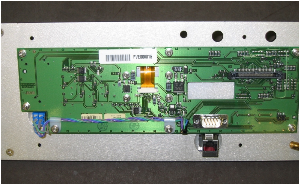
Figure 9.0-12 PAVE CCA Back
