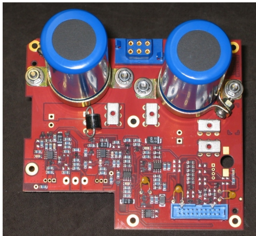
Figure 9.0-13 RALI CCA Top
