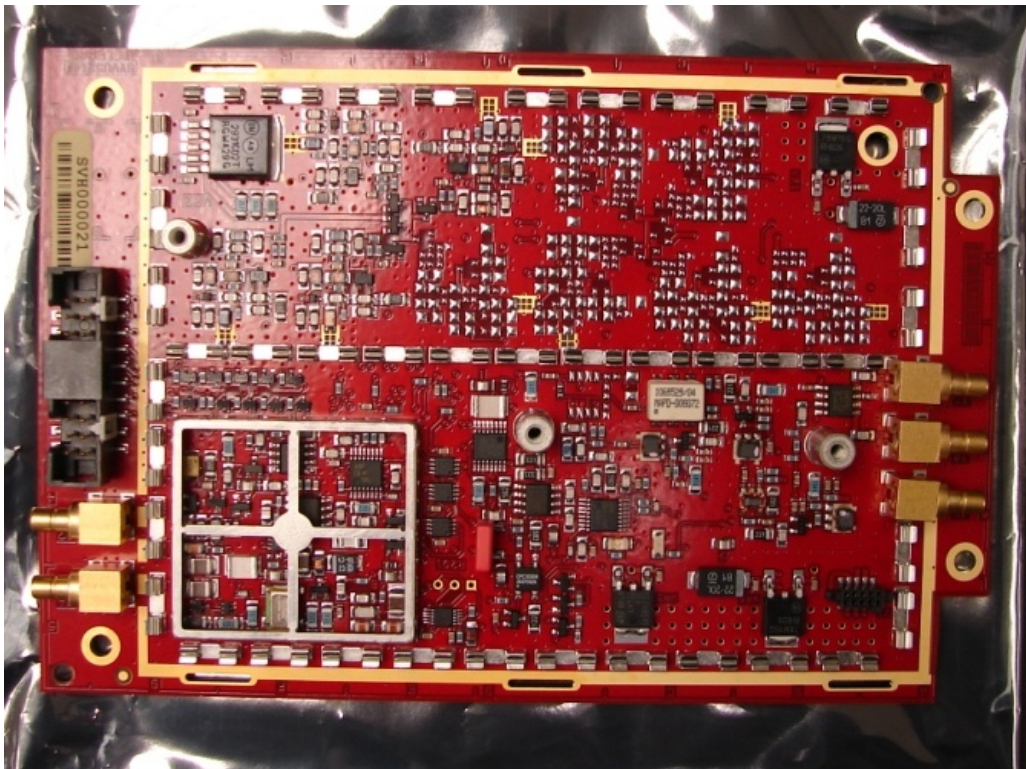
Figure 9.0-15 SVHF CCA Top
