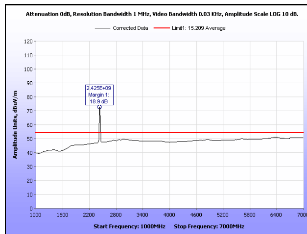
Plot 14. Radiated Spurious Emissions, Mid Channel, 1 GHz – 7 GHz, Average
