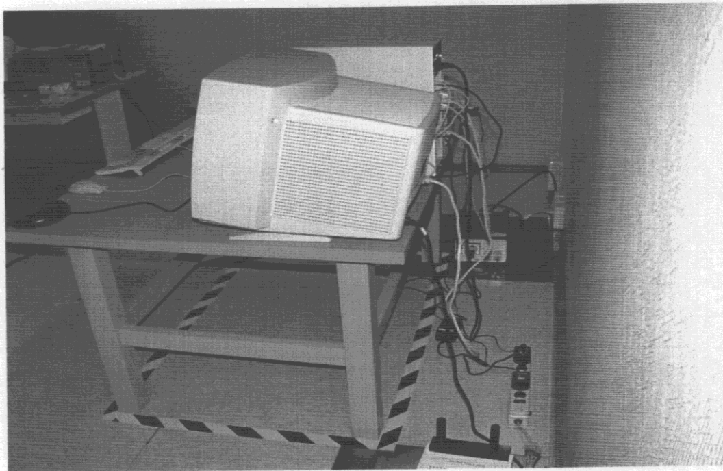
Back View of Conducted Test ( Maximum Testing Configuration)
