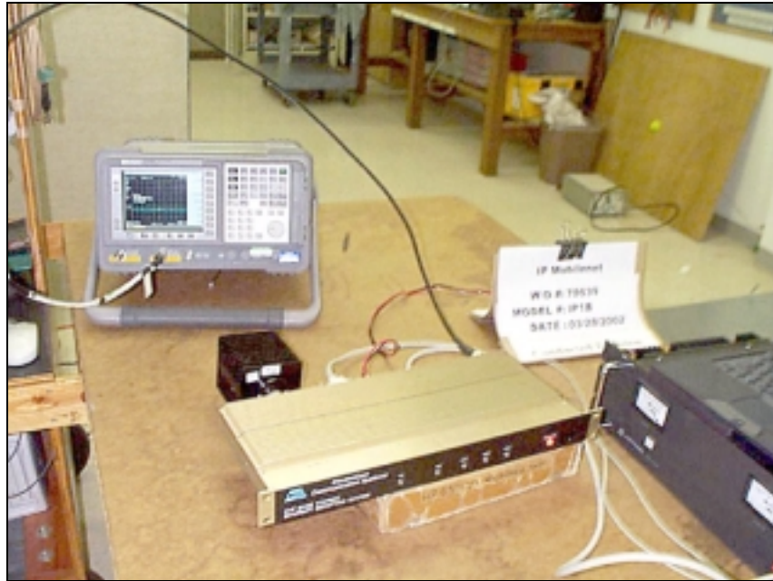
Antenna Power Conducted Emissions - Front View
