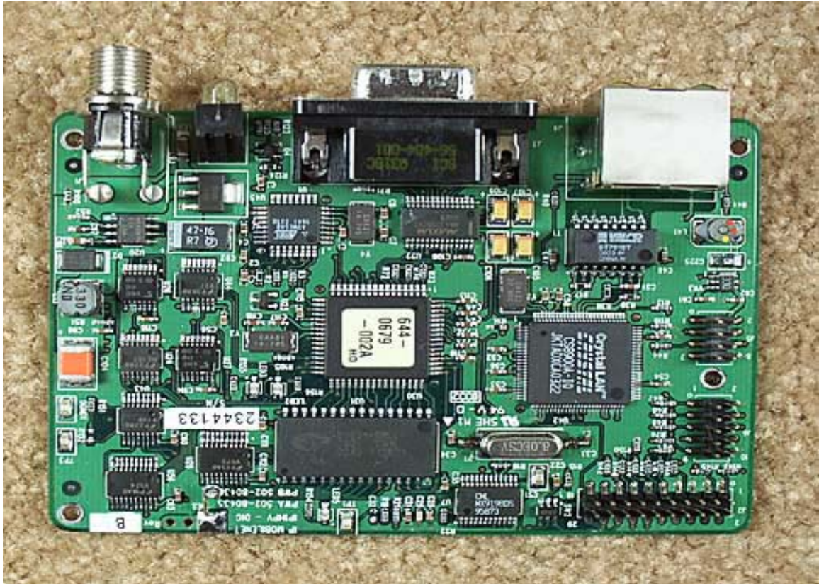
PCB 1 Top
