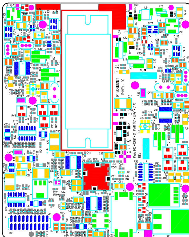
M32150-25 Mobile Radio RF Circuit Board
