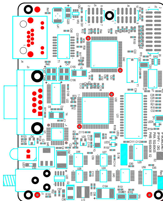
IP4 HPV Mobile Radio Digital Circuit Board
