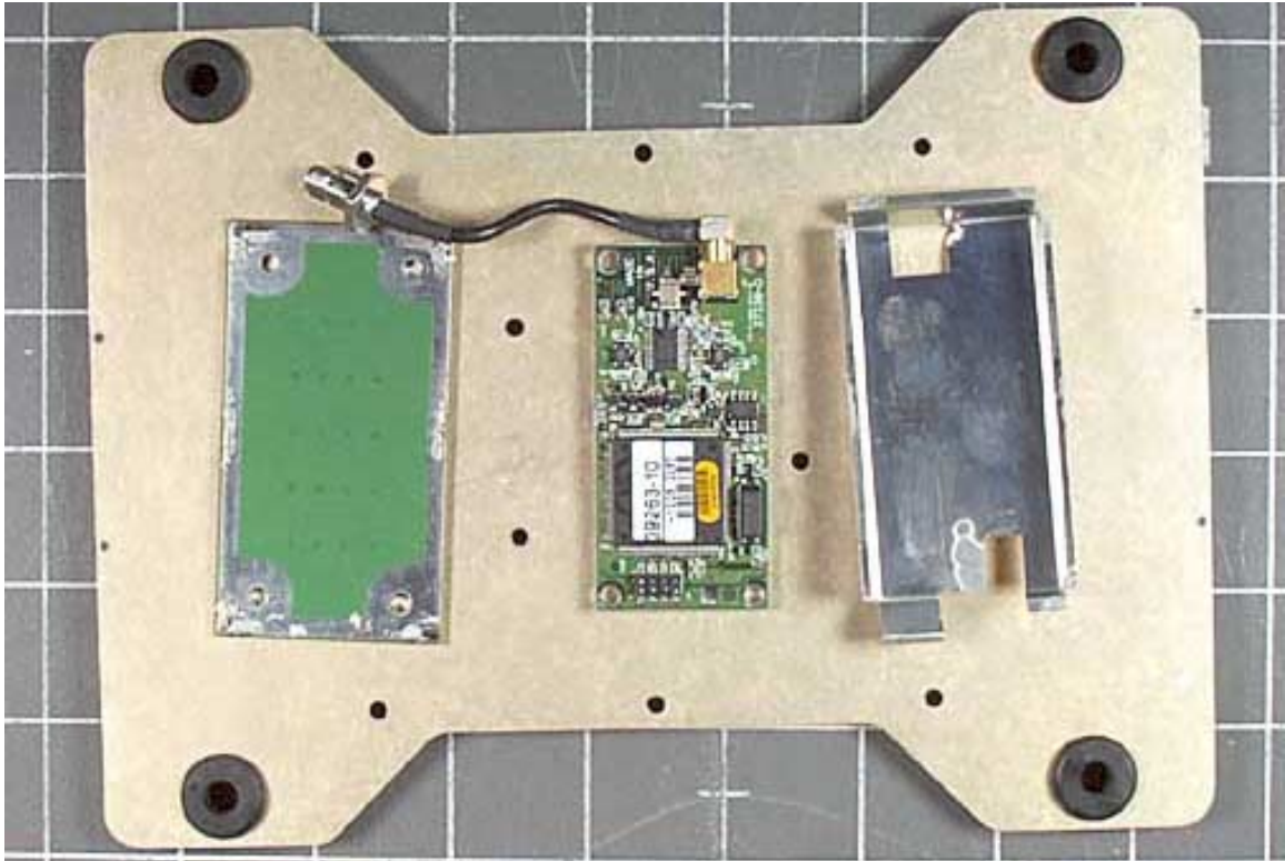
PCB 3 Shield Removed
