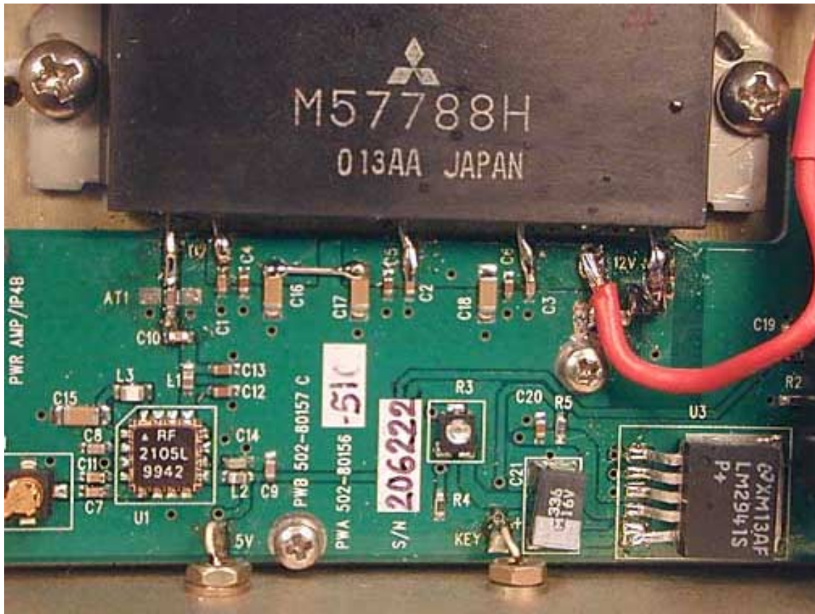
Power Amp – 451 MHz - Component
