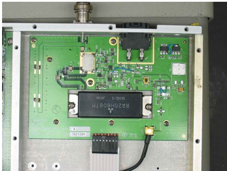
Amp Board
