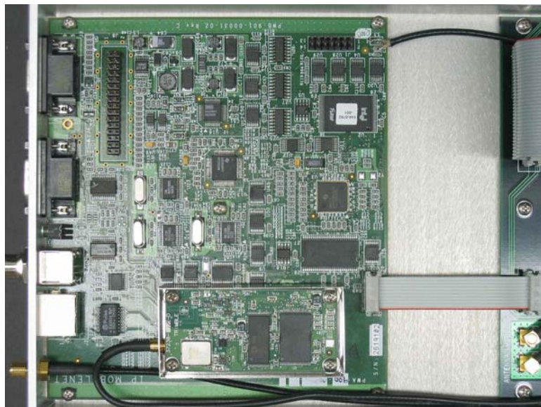
Base Station Internal View
