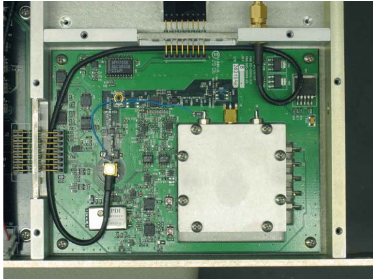
Exciter
