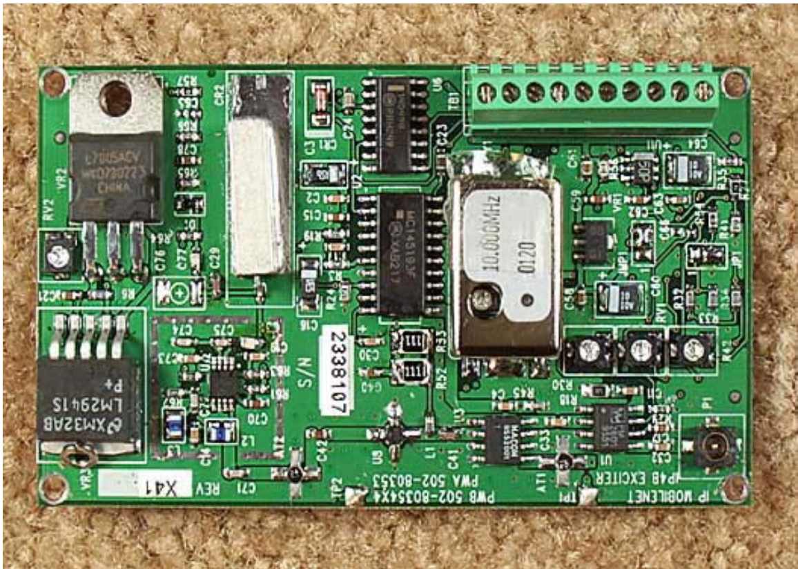
PCB TX Controller Top
