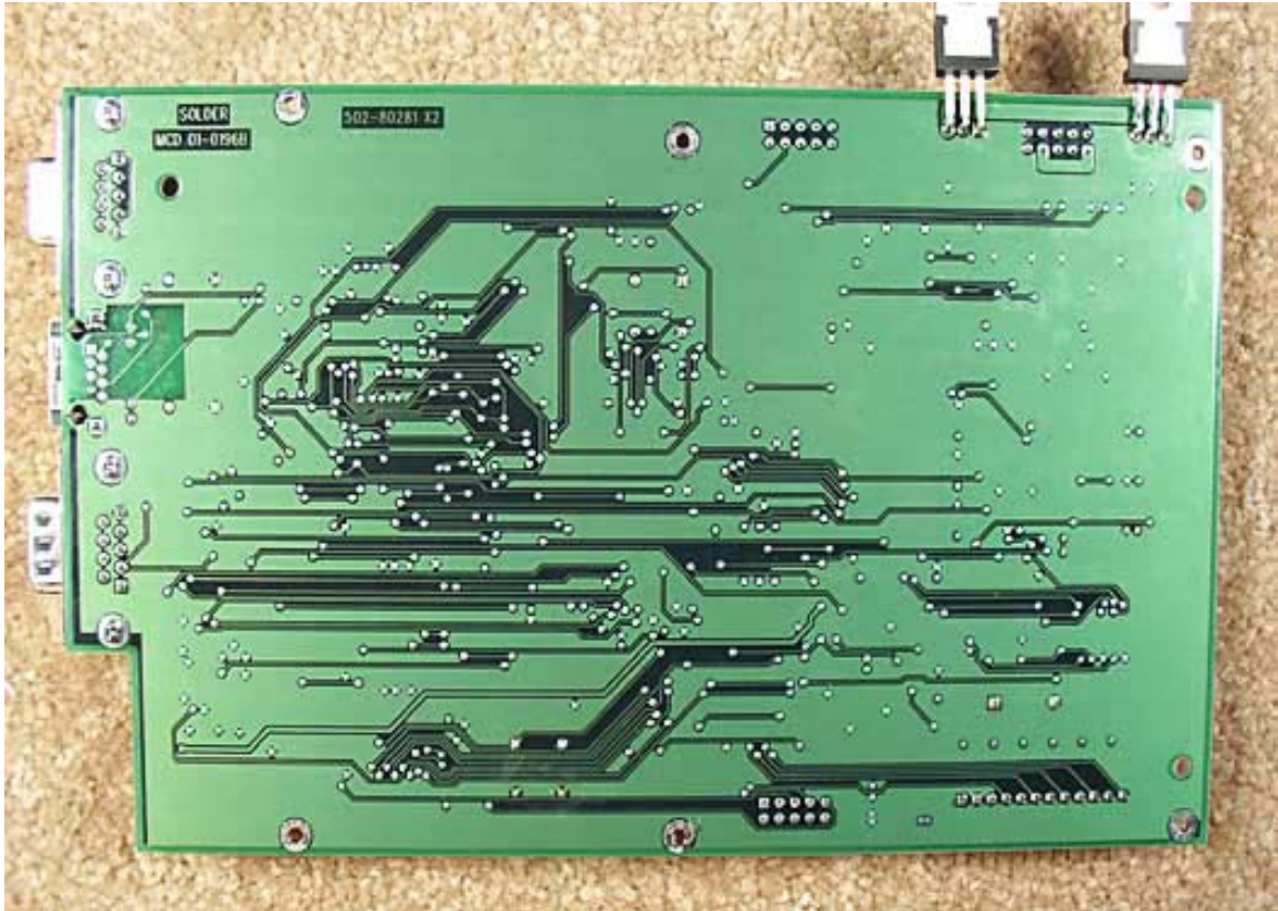
PCB Control Bottom All
