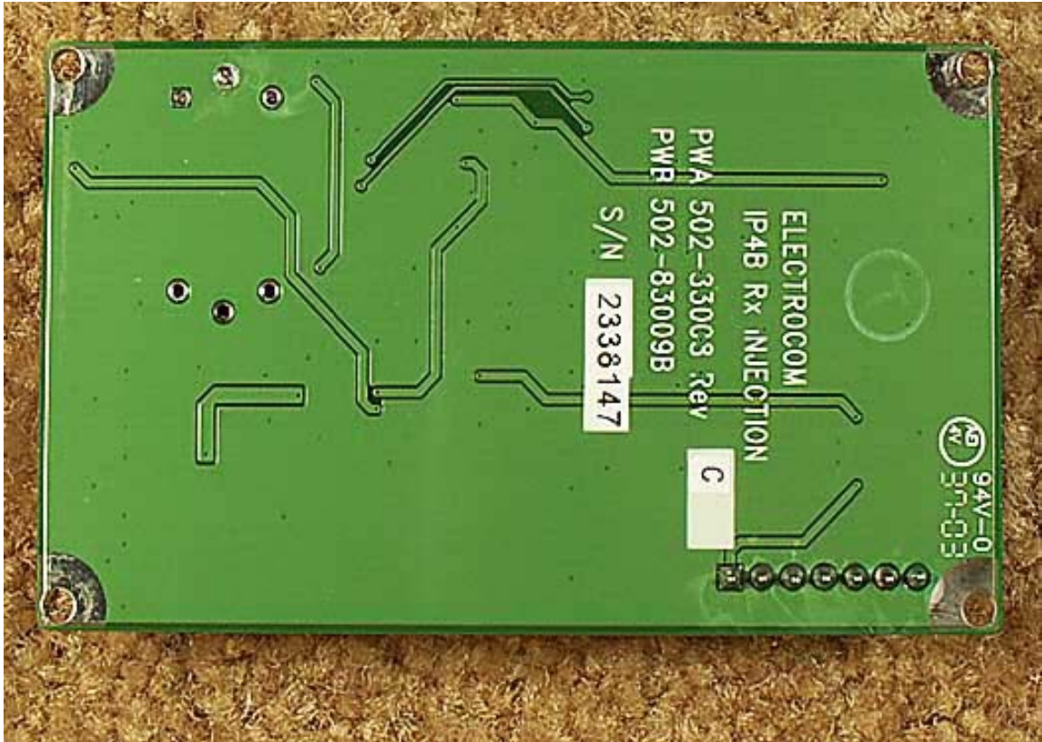
PCB RX Controller Bottom
