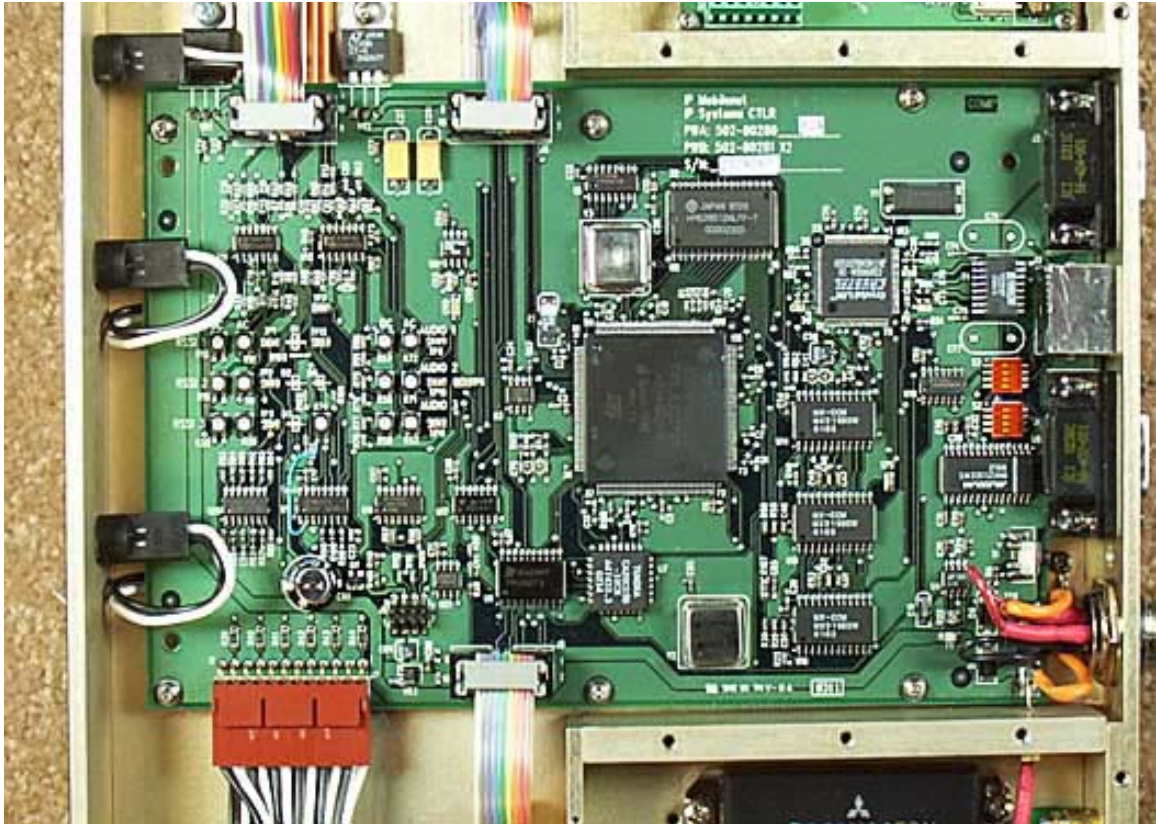
Internal Controller
