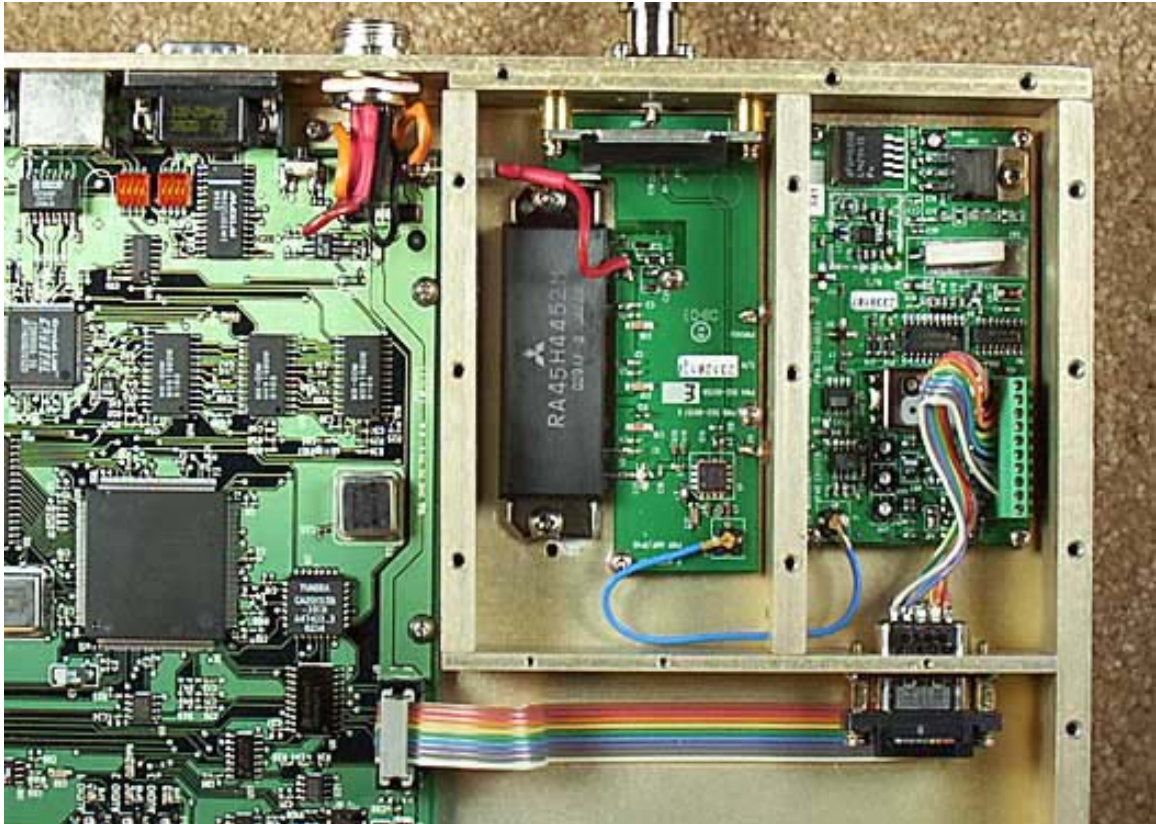
Internal TX
