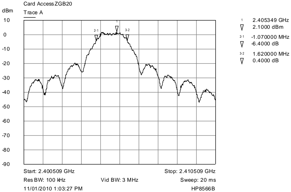
Trace A Lower channel bandwidth plot
