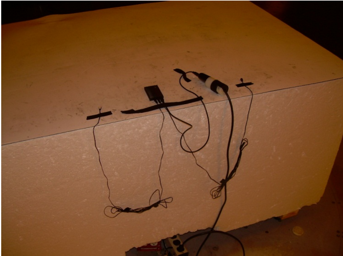
Photograph 2 – Back View Radiated Disturbance – Horizontal Configuration
