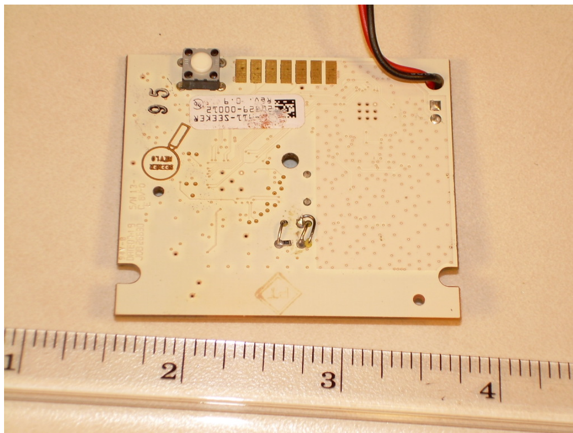
View of the Trace Side of the PCB - Internal Antenna
