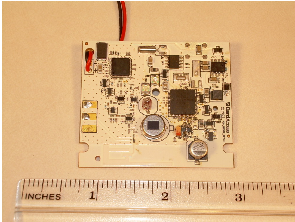
View of the Component Side of the PCB - Internal Antenna
