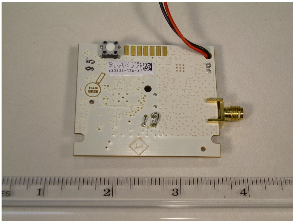
View of the Trace Side of the PCB - External Antenna
