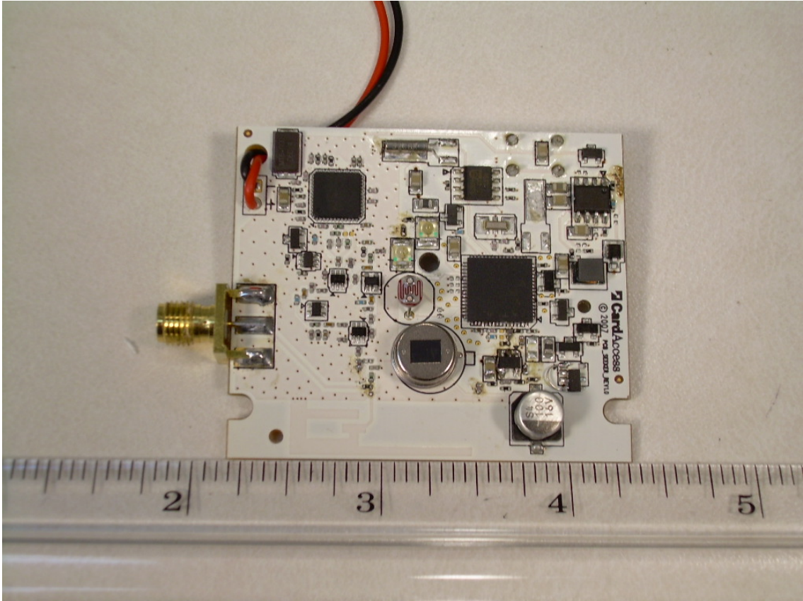
View of the Component Side of the PCB - External Antenna
