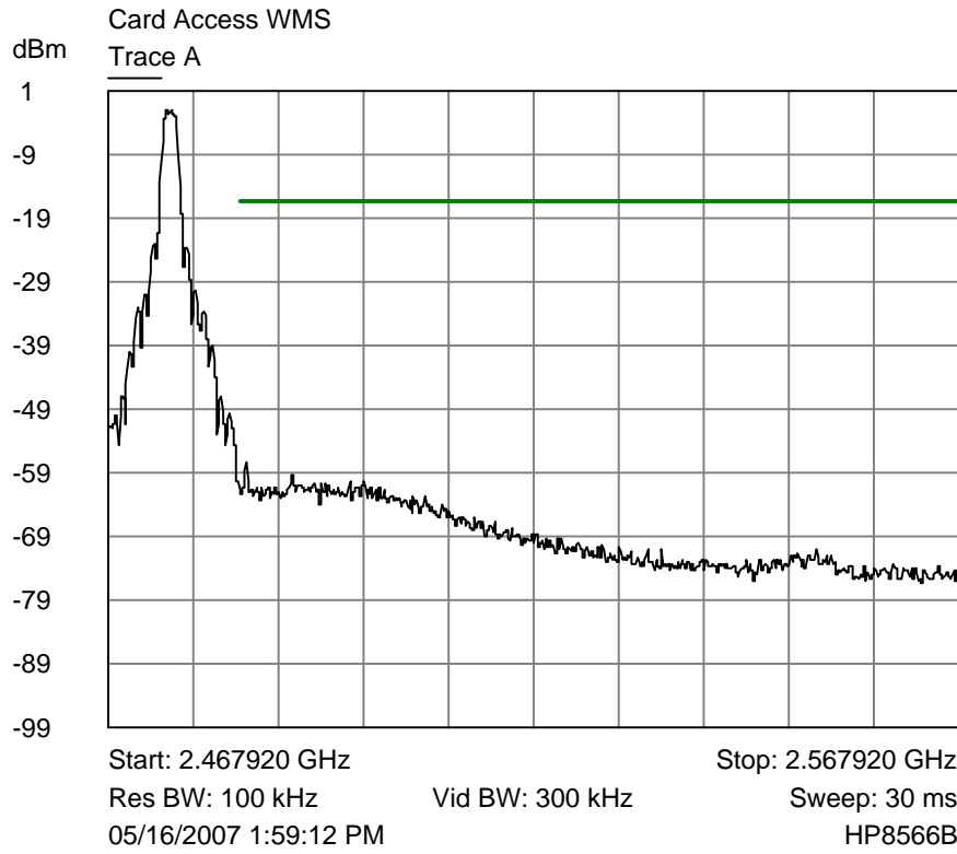
Trace A Upper channel band edge plot
