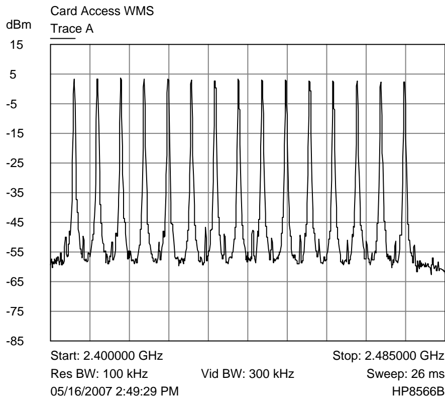
Trace A Channel plot, unmodulated carrier
