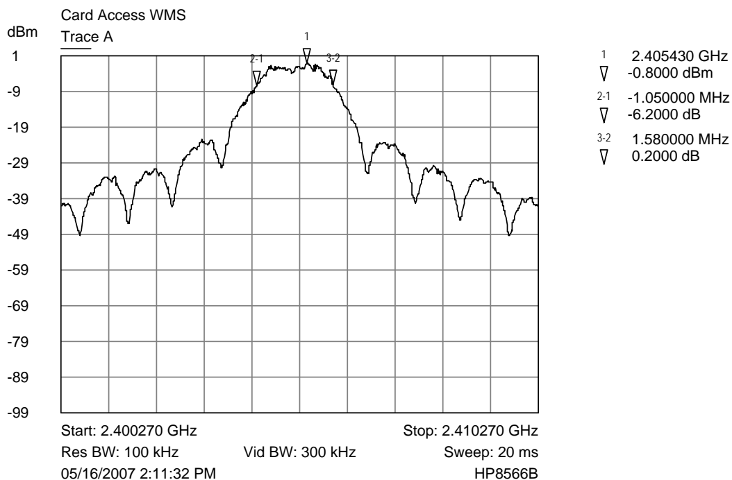
Trace A Lower channel bandwidth plot
