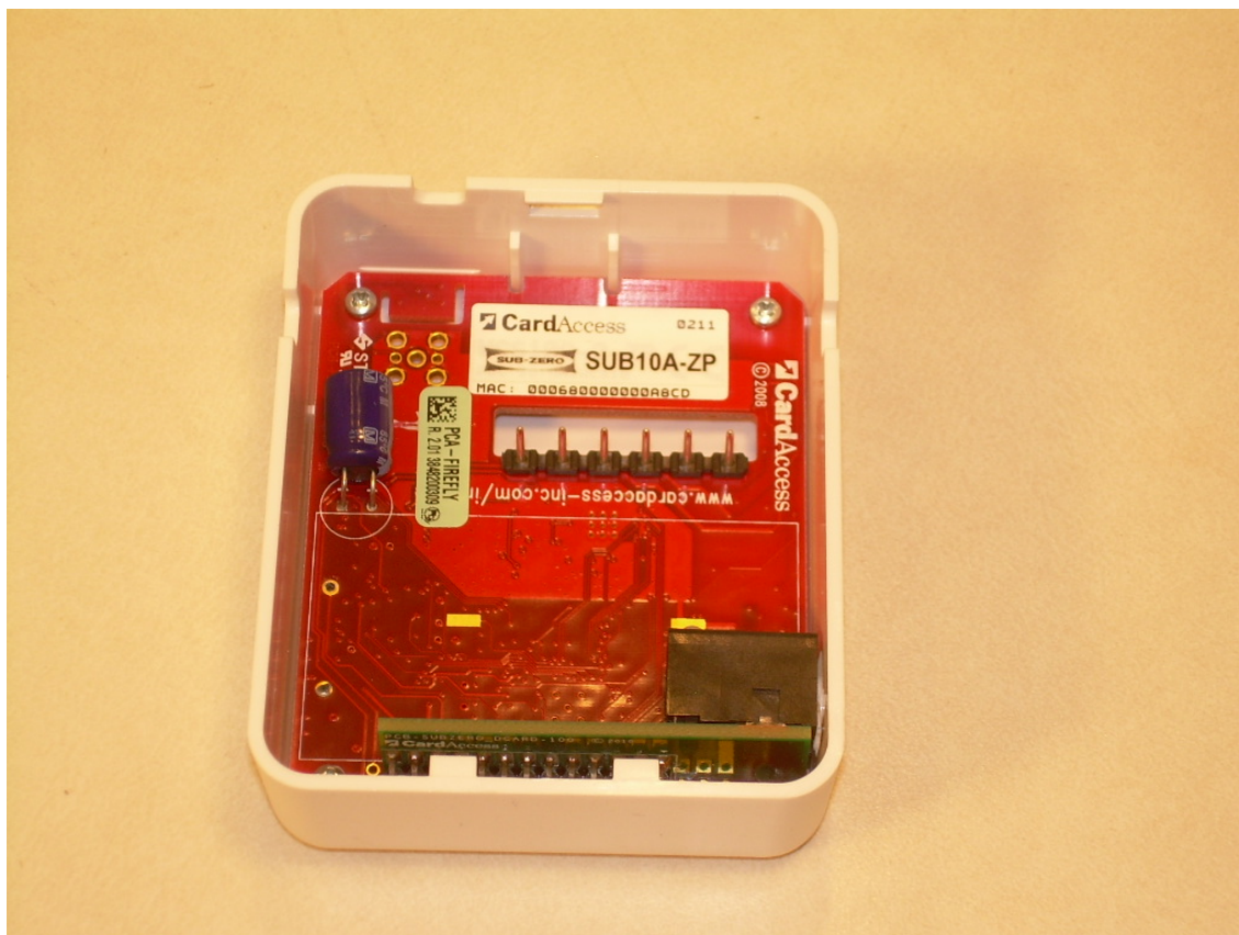
Internal View of the EUT – Back Housing Removed
