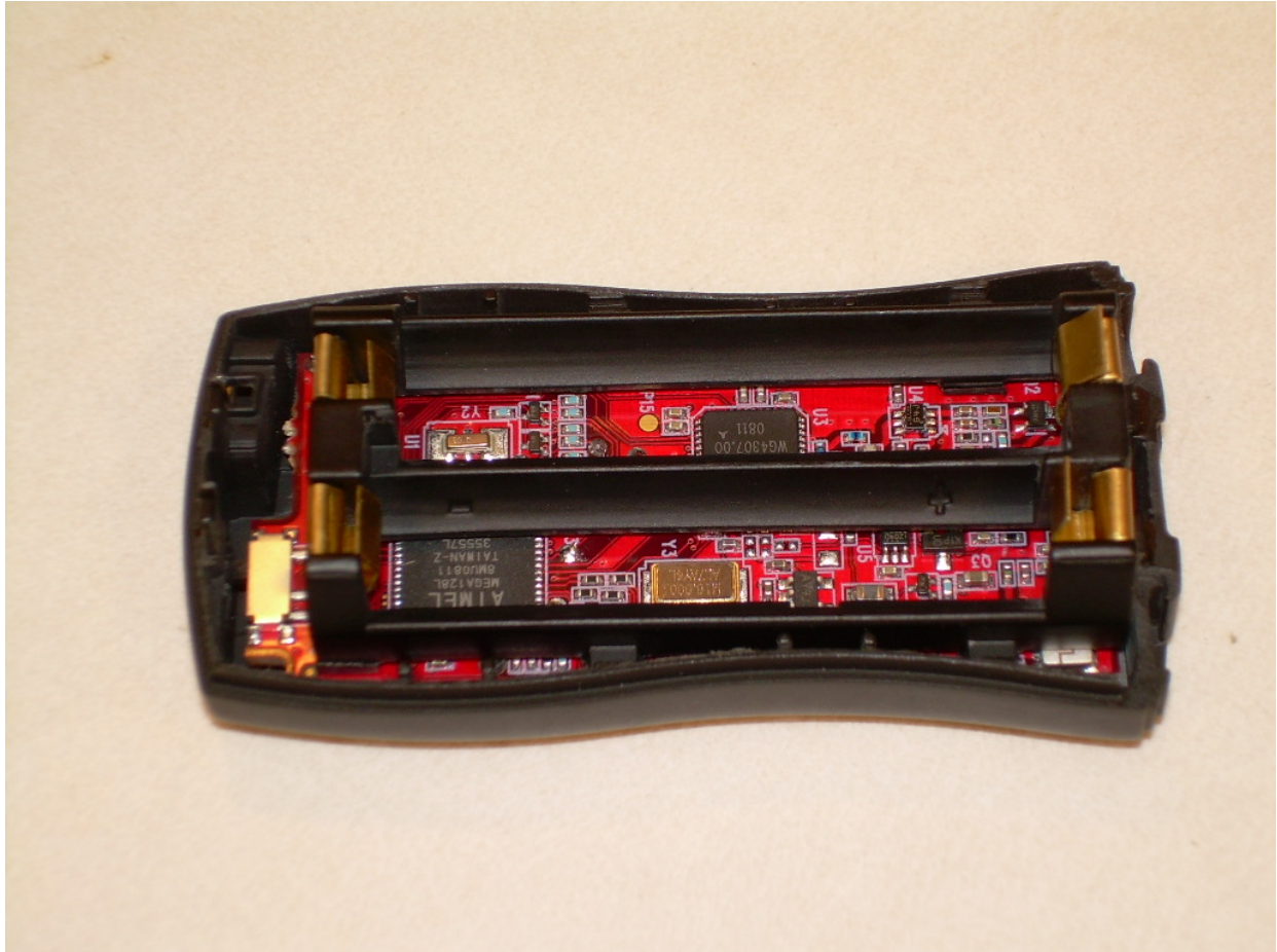
Photograph 4 - Internal View Front of the EUT
