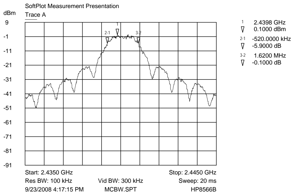
Trace A Middle channel band width
