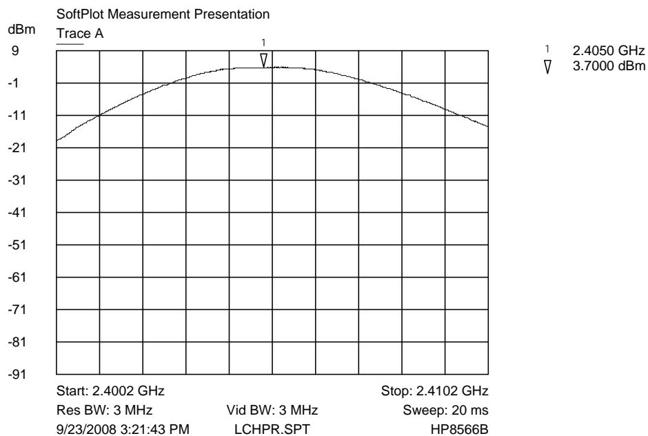
Trace A low channel Power
