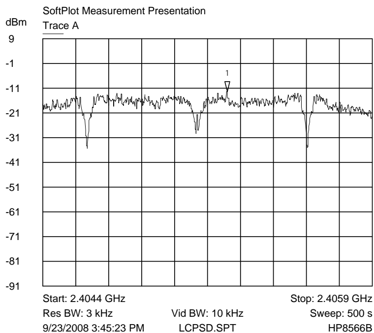
Trace A low channel 3 kHz power spectral density
