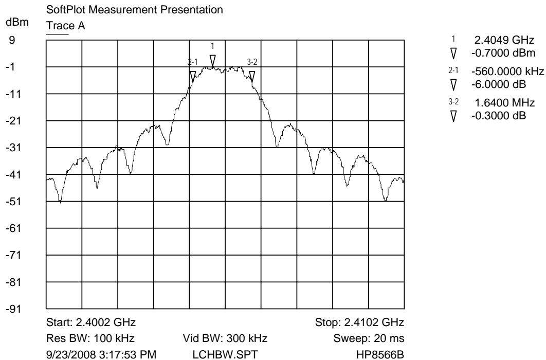
Trace A low channel bandwidth
