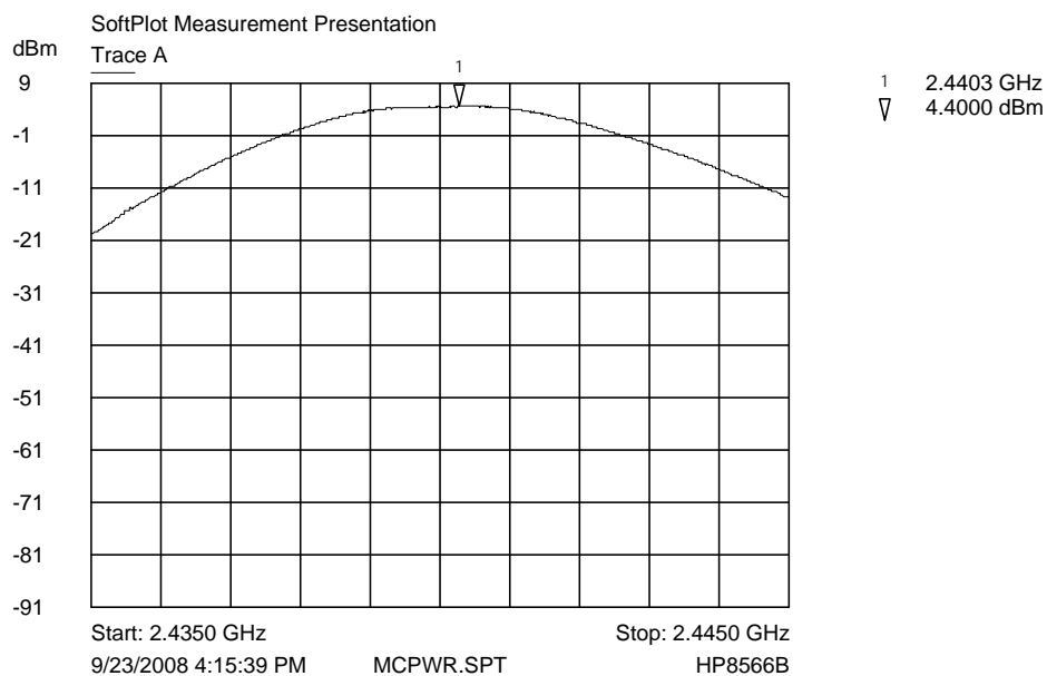
Trace A Middle channel output power
