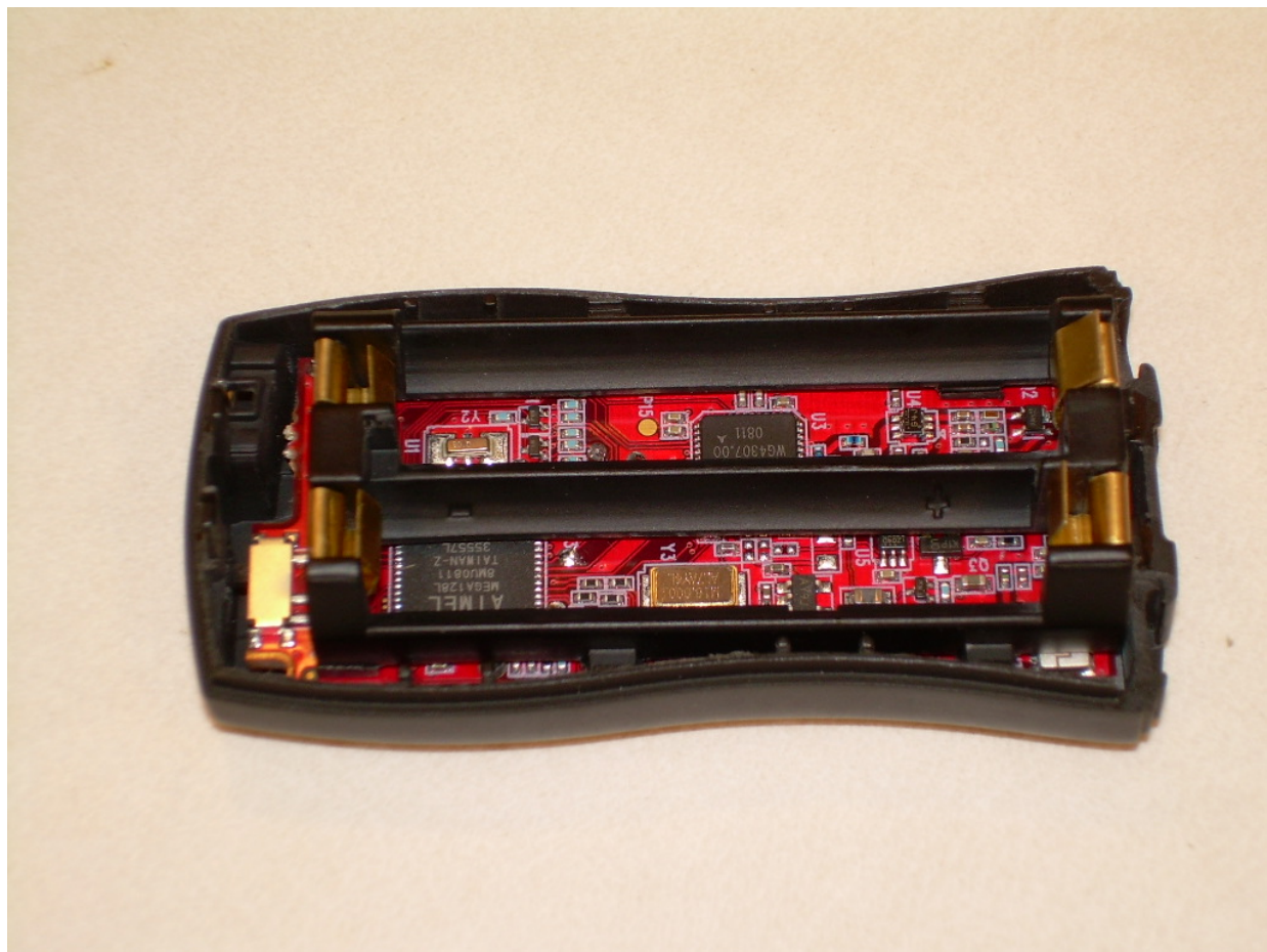
Internal View Front of the EUT
