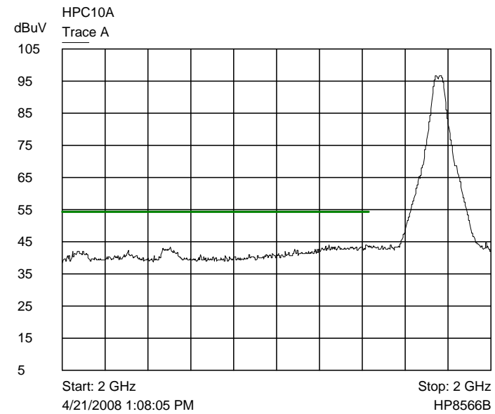
Trace A lower channel band edge - radiated
