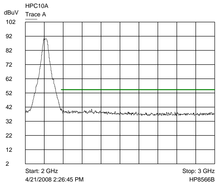
Trace A upper channel band edge - radiated
