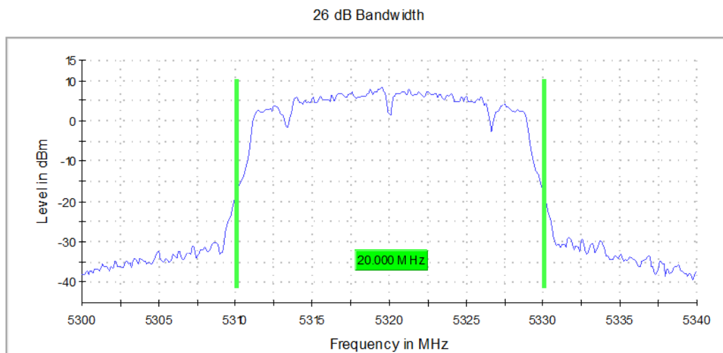
Graph 3: 26 dB Emissions Bandwidth Transmitting at 5320 MHz
