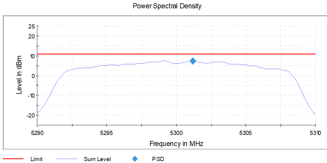
Graph 14: Power Spectral Density Transmitting at 5300 MHz
