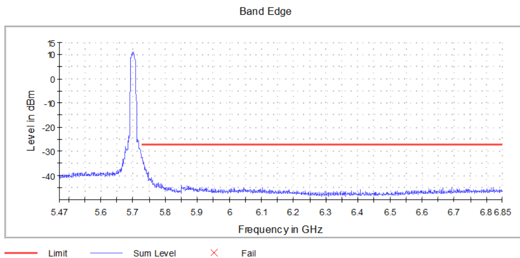
Graph 24: High Band Edge Channel 140 Transmitting (5700 MHz)
