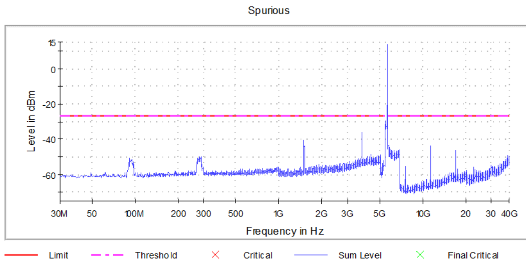
Graph 30: Spurious Emissions Channel 140 Transmitting (5700 MHz)
