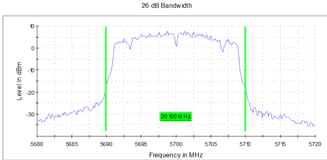
Graph 6: 26 dB Emissions Bandwidth Transmitting at 5700 MHz
