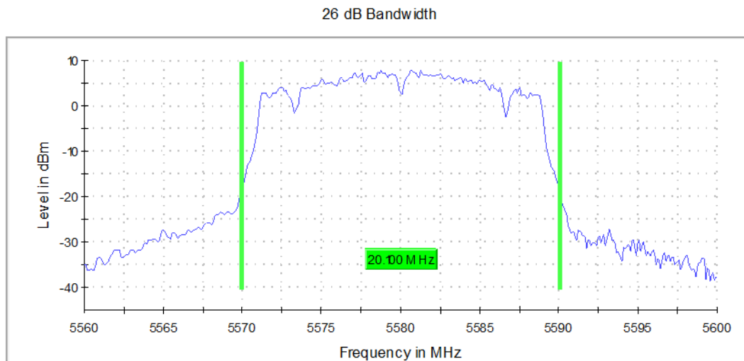
Graph 5: 26 dB Emissions Bandwidth Transmitting at 5580 MHz
