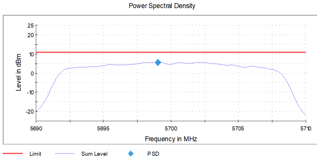
Graph 18: Power Spectral Density Transmitting at 5700 MHz
