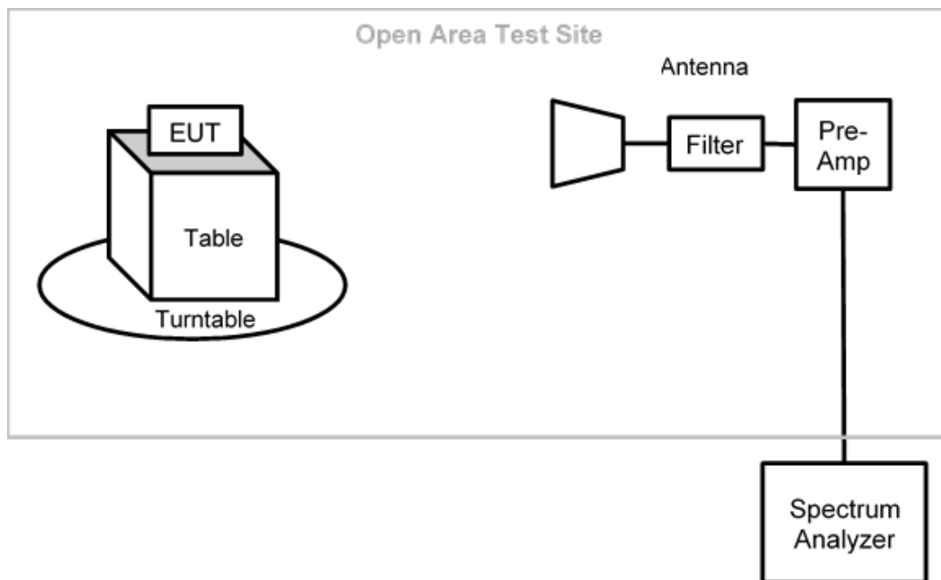
Figure 34: Radiated Emissions Above 1GHz Test
