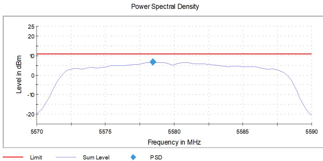
Graph 17: Power Spectral Density Transmitting at 5580 MHz
