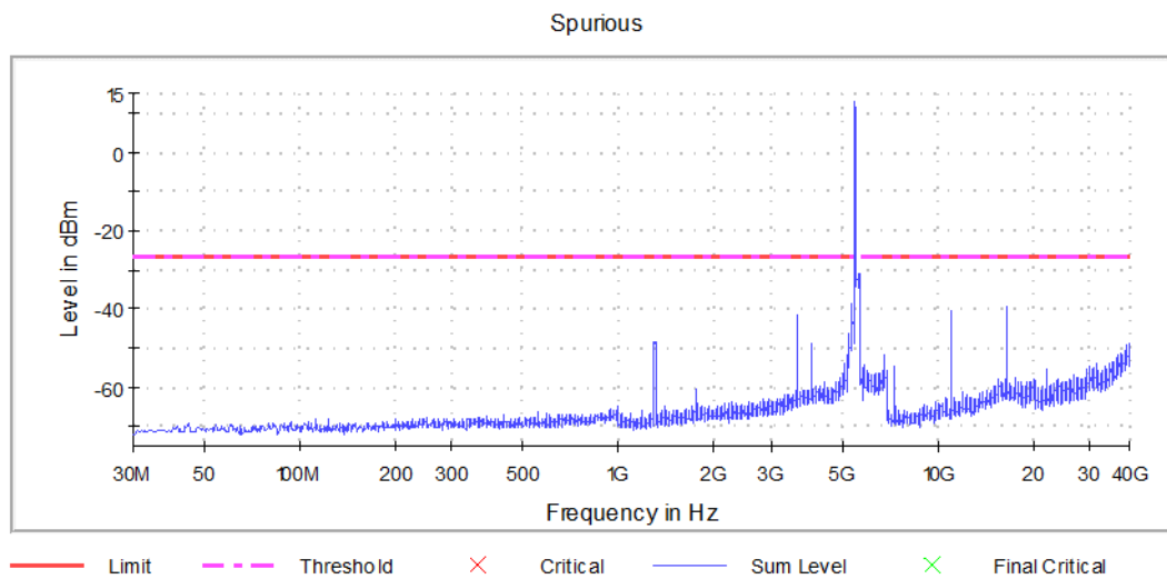
Graph 28: Spurious Emissions Channel 100 Transmitting (5500 MHz)
