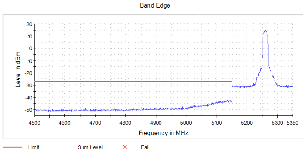
Graph 21: Low Band Edge Channel 52 Transmitting (5260 MHz)
