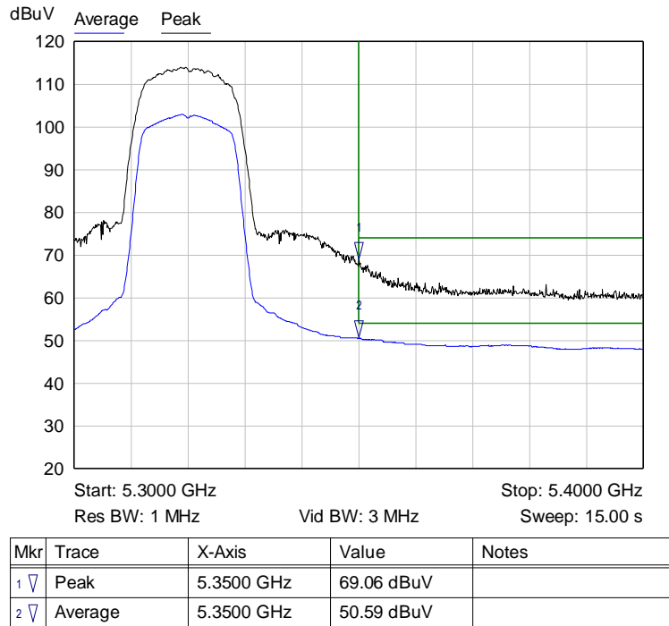
Graph 19: Channel 64 Band Edge at the Restricted Band Plot
