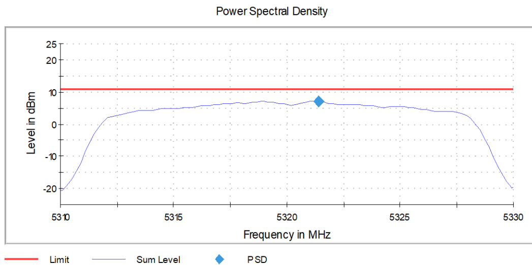
Graph 15: Power Spectral Density Transmitting at 5320 MHz
