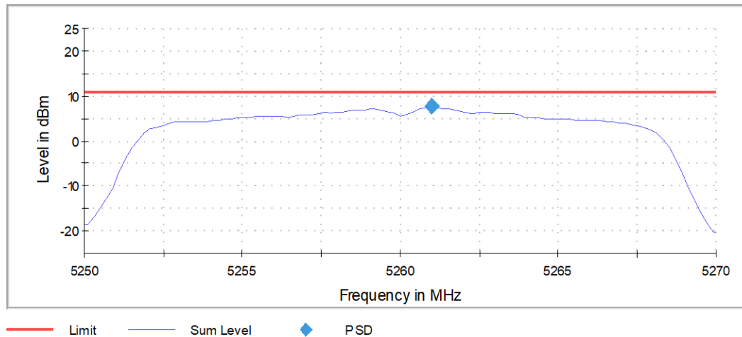
Graph 13: Power Spectral Density Transmitting at 5260 MHz
