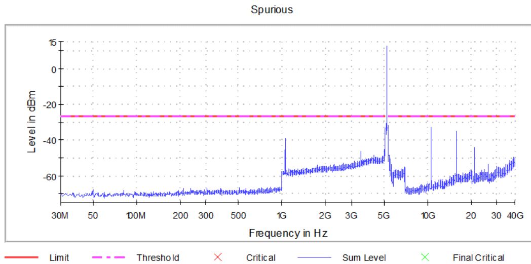
Graph 25: Spurious Emissions Channel 52 Transmitting (5260 MHz)
