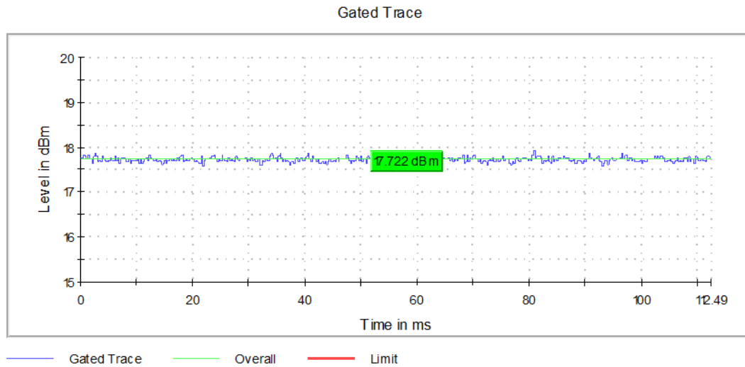
Graph 7: Output Power Transmitting at 5260 MHz
