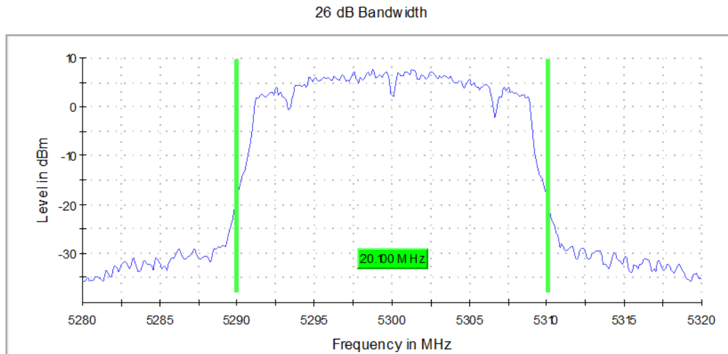
Graph 2: 26 dB Emissions Bandwidth Transmitting at 5300 MHz
