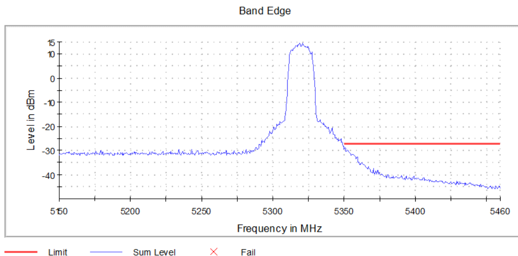
Graph 22: High Band Edge Channel 64 Transmitting (5320 MHz)
