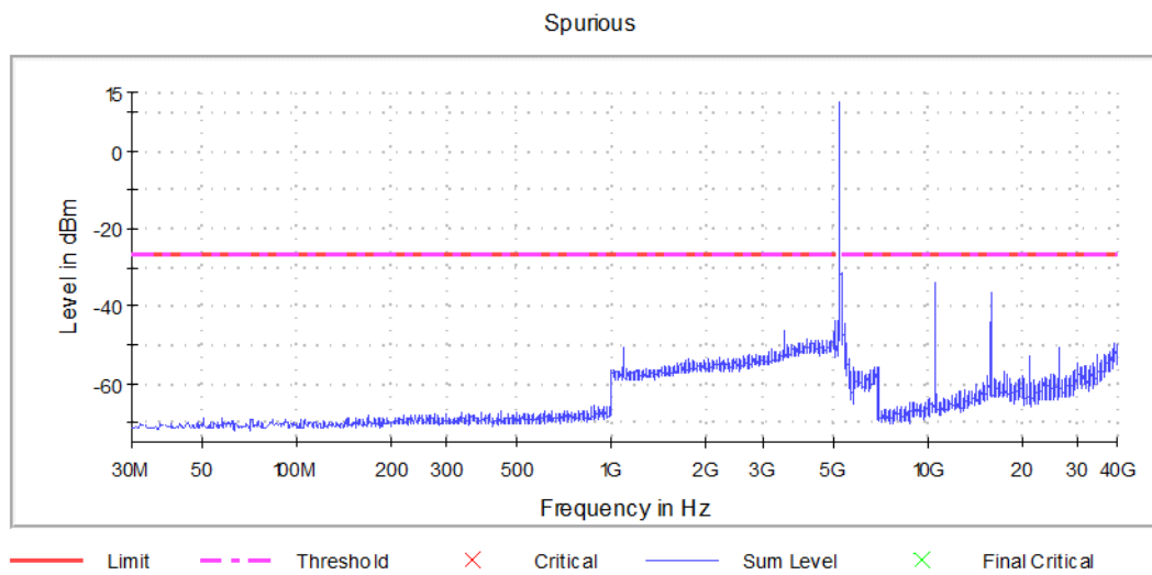
Graph 26: Spurious Emissions Channel 60 Transmitting (5300 MHz)
