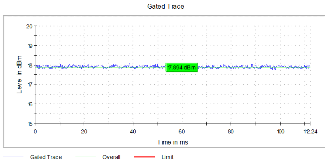
Graph 8: Output Power Transmitting at 5300 MHz
