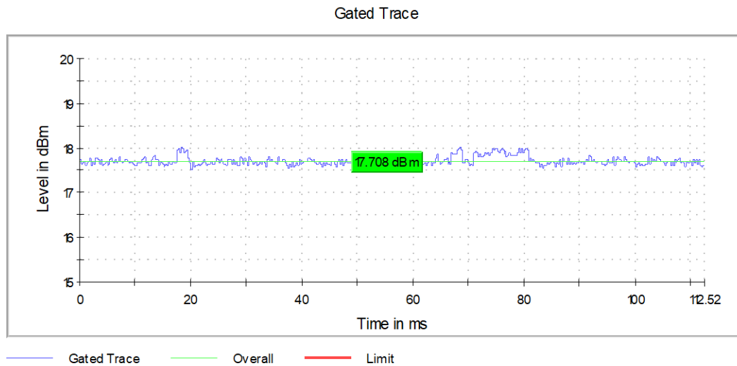
Graph 11: Output Power Transmitting at 5580 MHz
