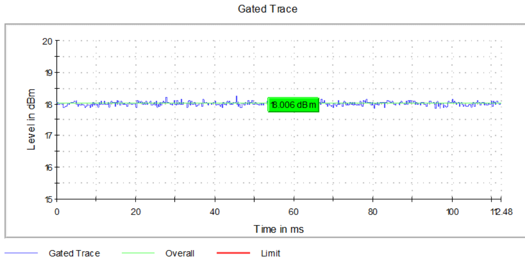
Graph 9: Output Power Transmitting at 5320 MHz
