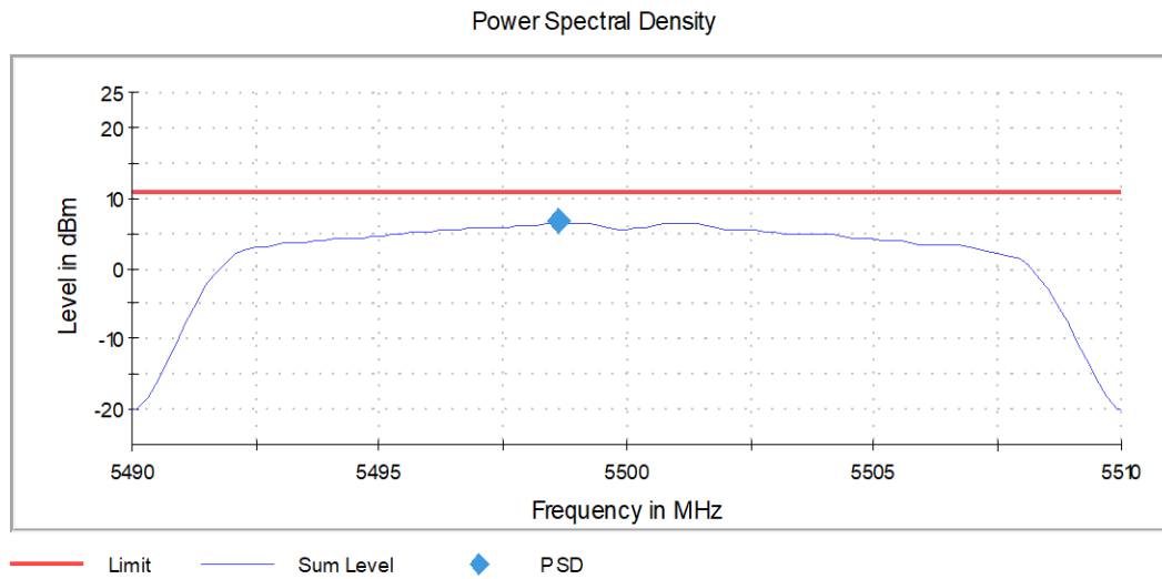
Graph 16: Power Spectral Density Transmitting at 5500 MHz
