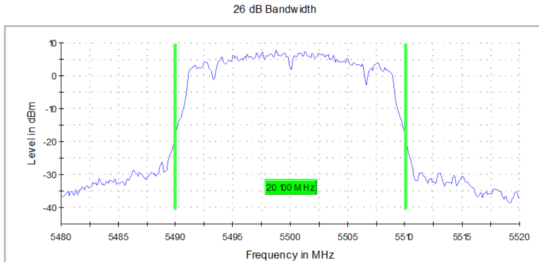
Graph 4: 26 dB Emissions Bandwidth Transmitting at 5500 MHz
