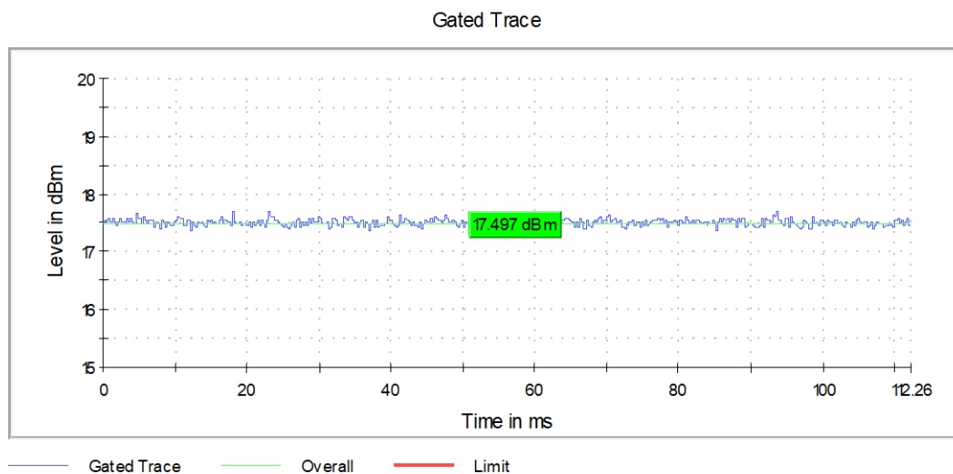
Graph 12: Output Power Transmitting at 5700 MHz
