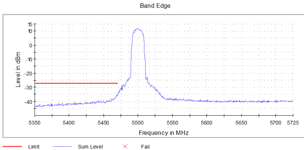
Graph 23: Low Band Edge Channel 100 Transmitting (5500 MHz)
