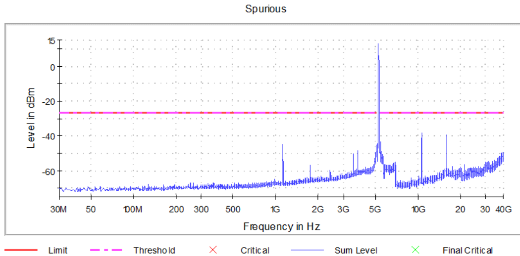
Graph 27: Spurious Emissions Channel 64 Transmitting (5320 MHz)
