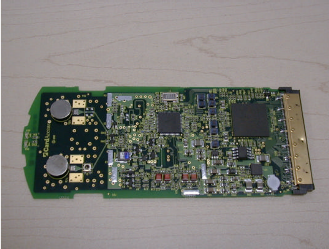
Top PCB:
