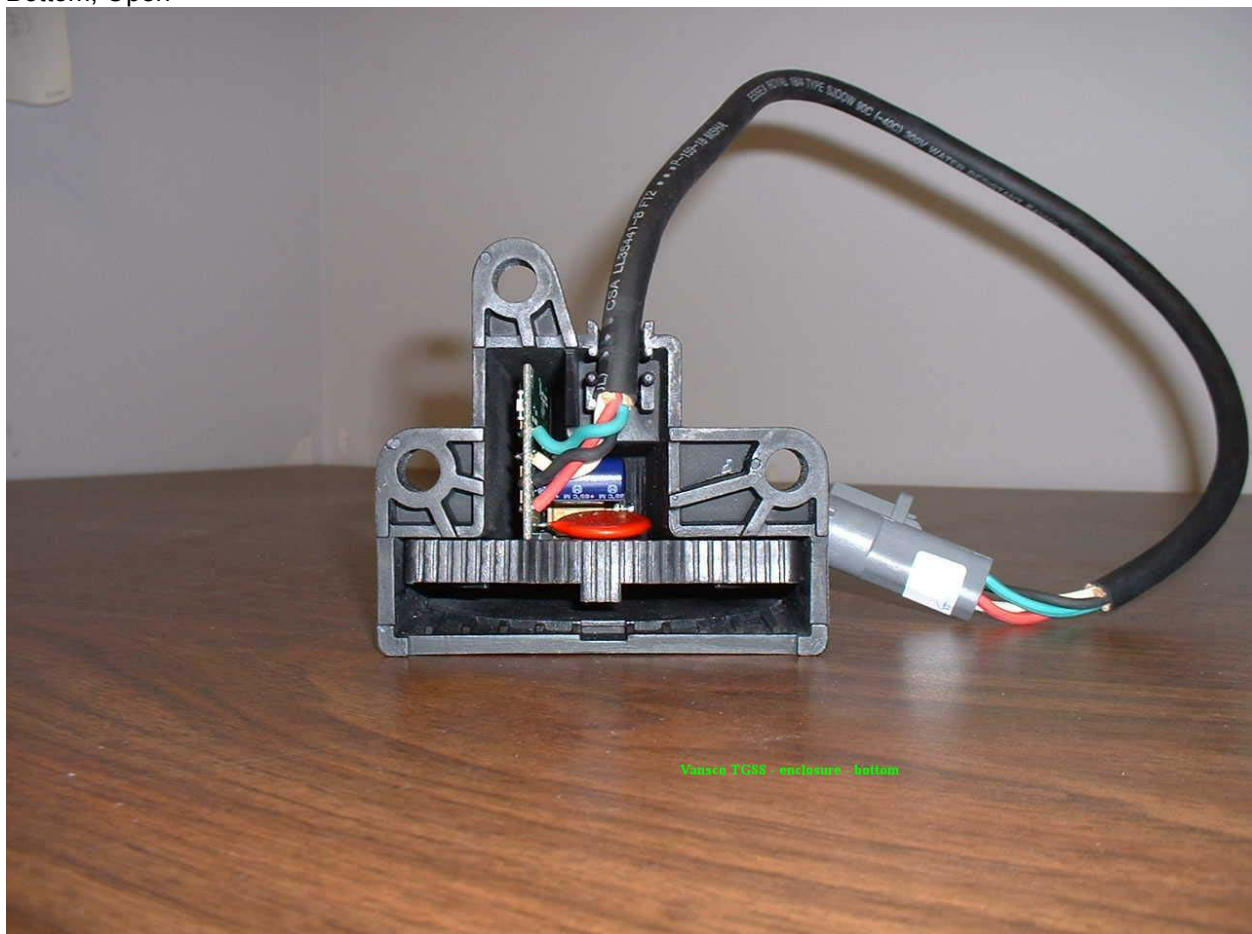
Bottom, Open
