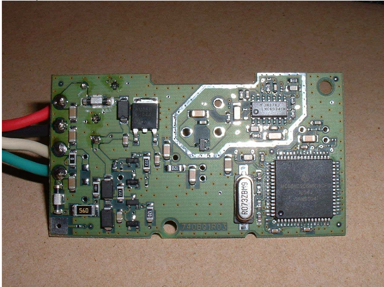
Board Top
