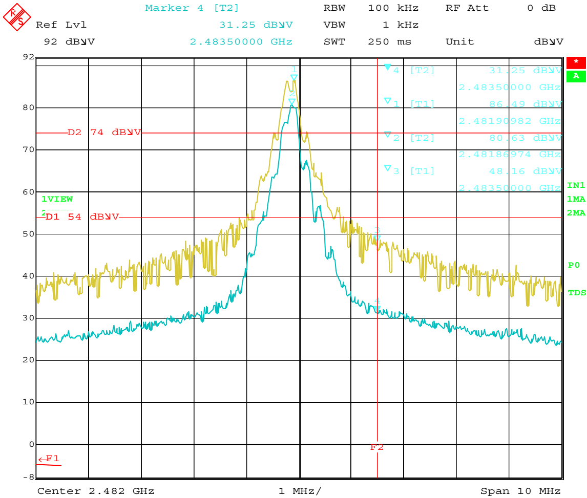
Band Edge – High Channel – Horizontal Polarization – Z-Axis (Worst Case)
