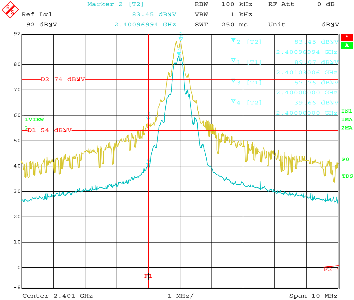
Band Edge – Low Channel – Vertical Polarization – Z-Axis (Worst Case)
