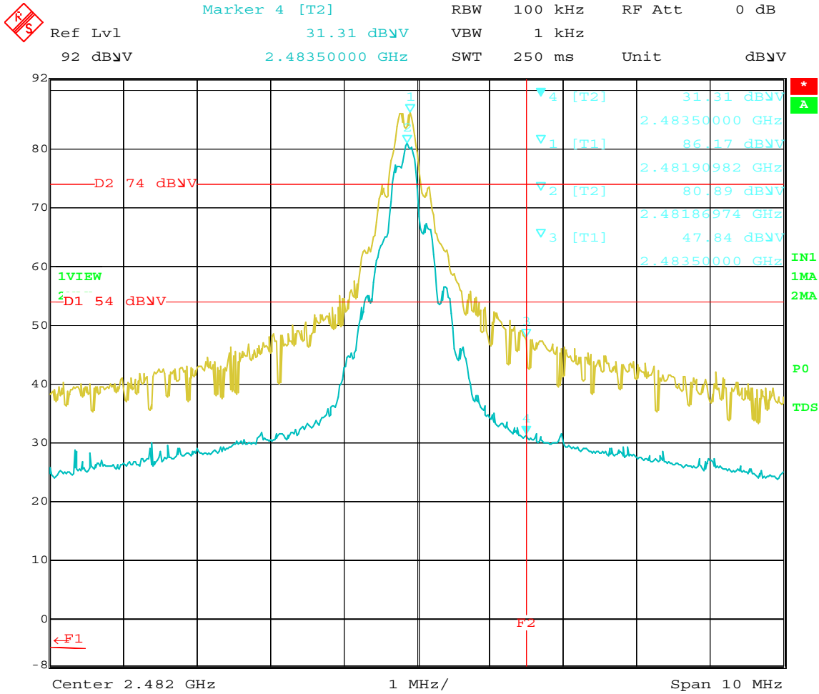
Band Edge – High Channel – Vertical Polarization – Z-Axis (Worst Case)
