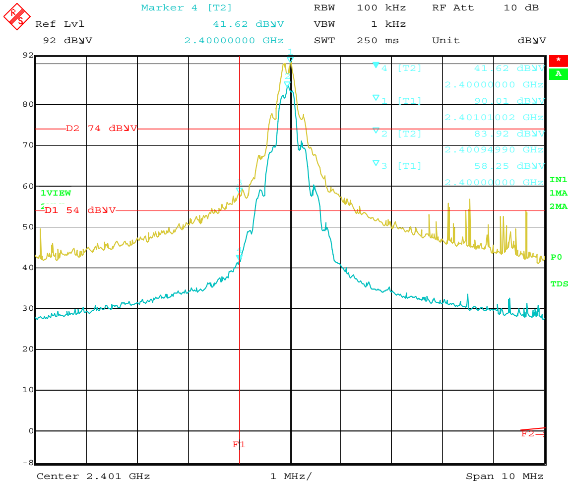
Band Edge – Low Channel – Horizontal Polarization – X-Axis (Worst Case)
