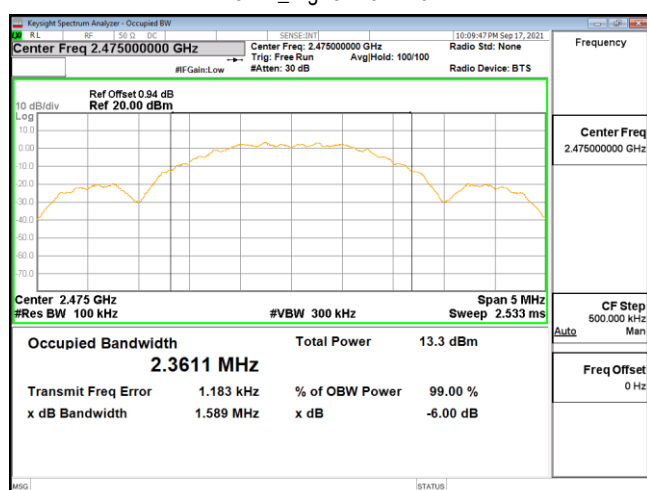
OBW_HighCH25-2475
