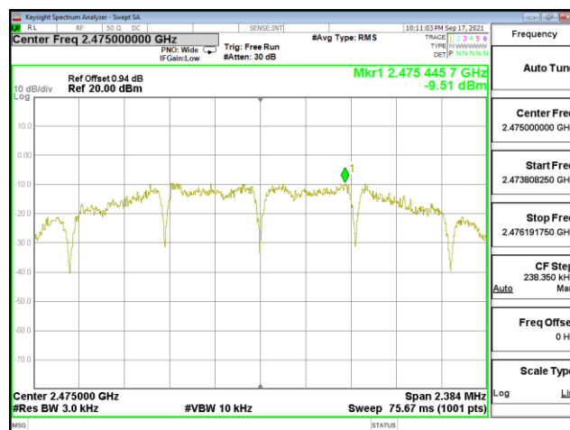
PSD_HighCH25-2475
