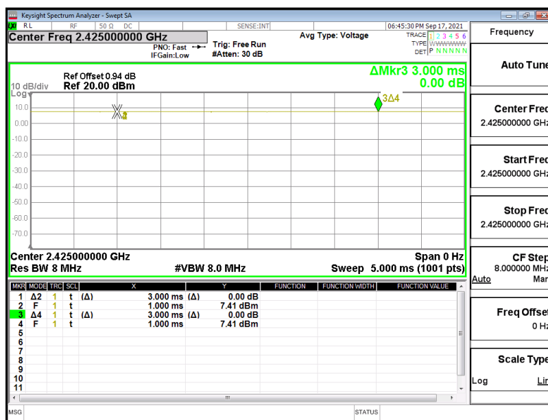
Zigbee_1M_LowCH15-2425
