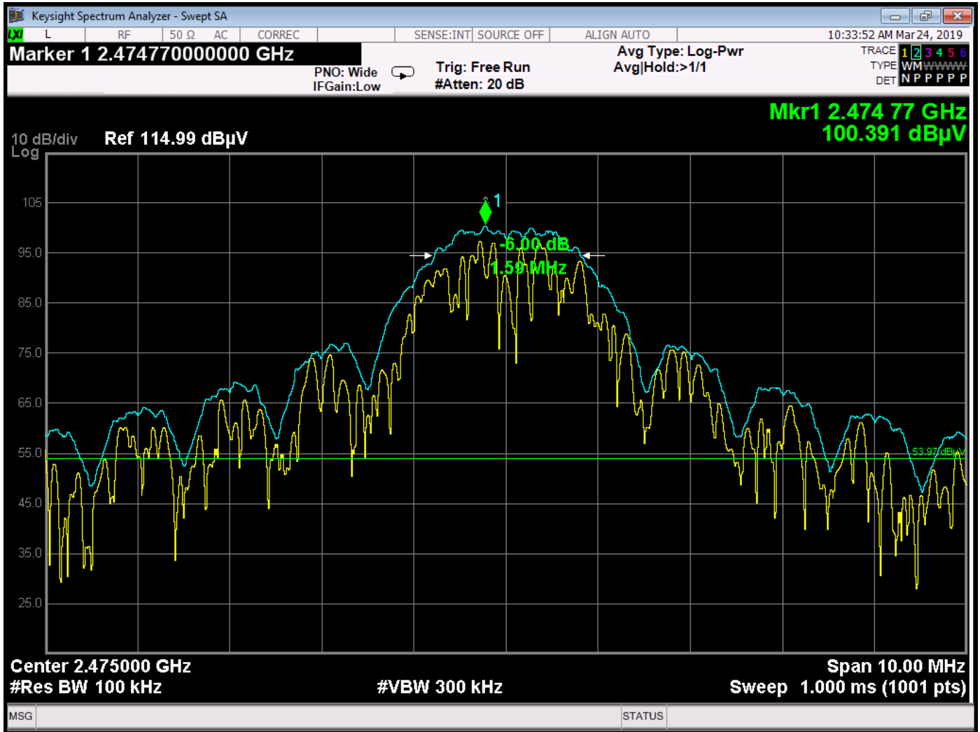
Bandwidth 6 dB - 2475 MHz
