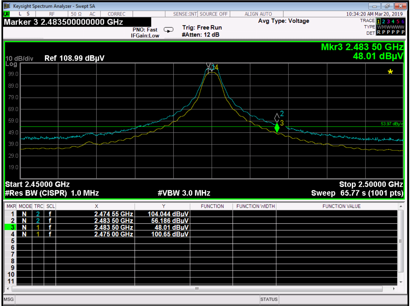
BE - 2475 MHz - Horizontal - X-Axis Worst Case – RF4CE Mode
