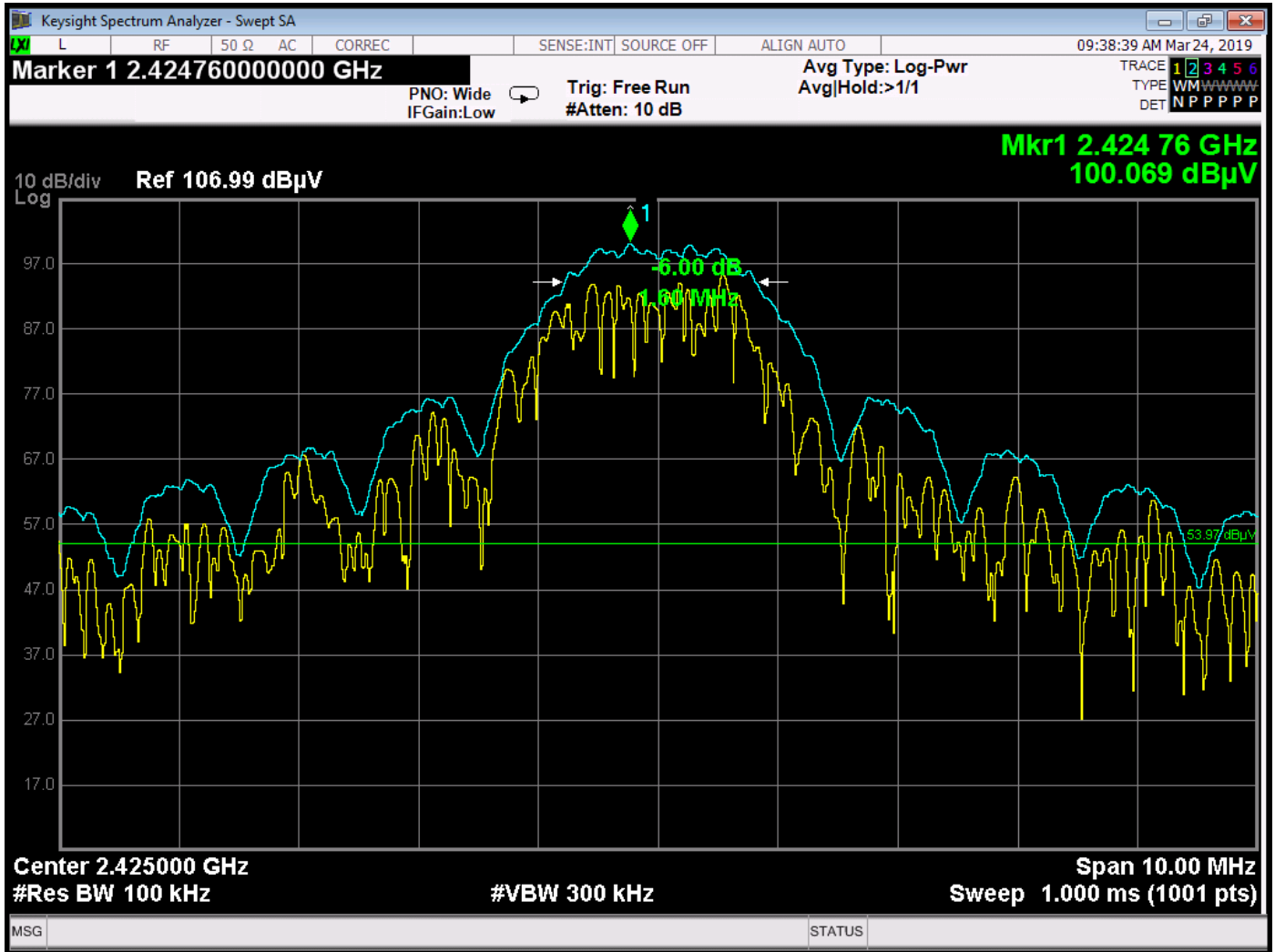
Bandwidth 6 dB - 2425 MHz
