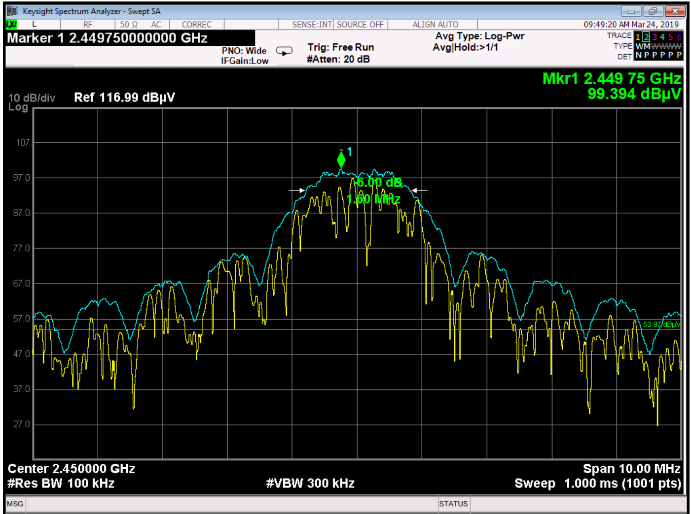
Bandwidth 6 dB - 2450 MHz
