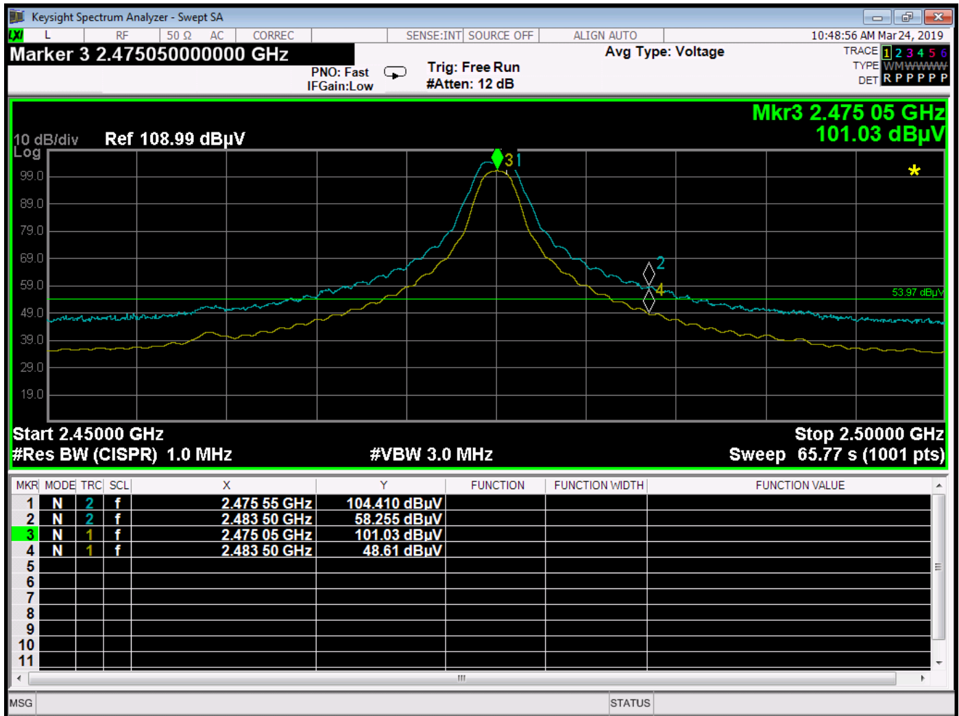
BE - 2475 MHz - Vertical - Y-Axis Worst Case – RF4CE Mode
