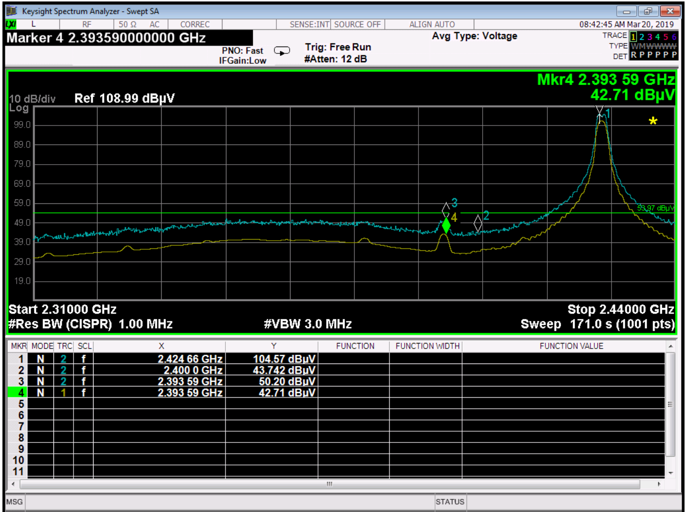
BE - 2425 MHz - Horizontal - X-Axis Worst Case – RF4CE Mode
