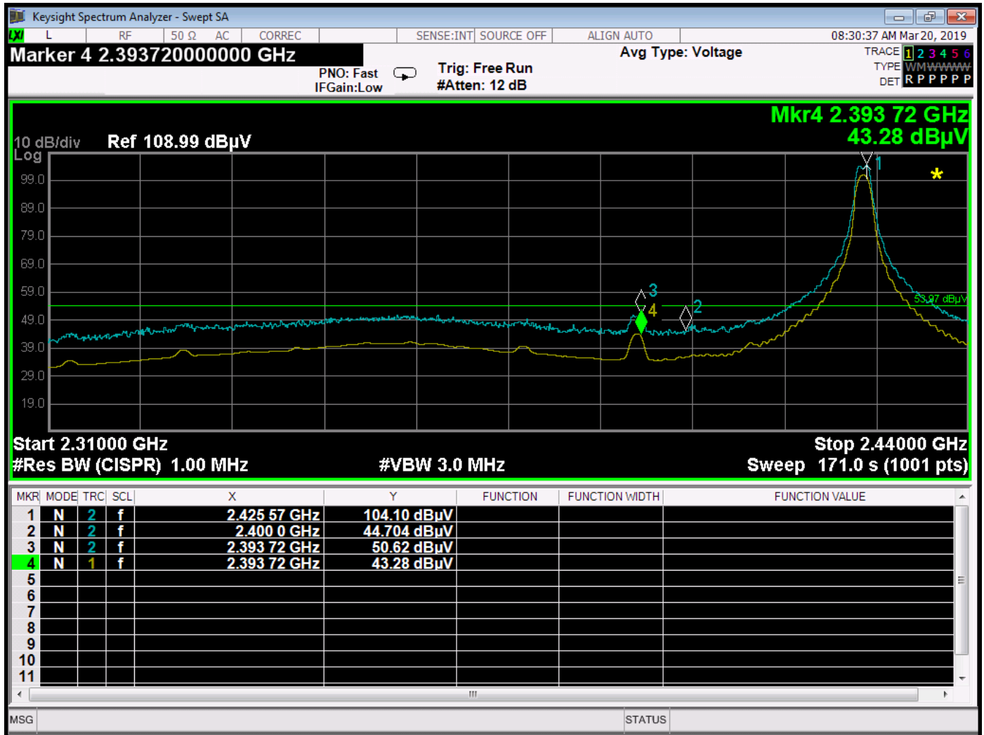
BE - 2425 MHz - Vertical - Y-Axis Worst Case – RF4CE Mode
