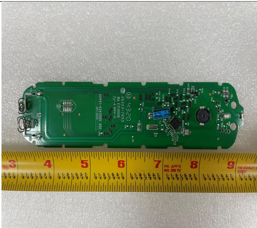
EUT Internal-Back
