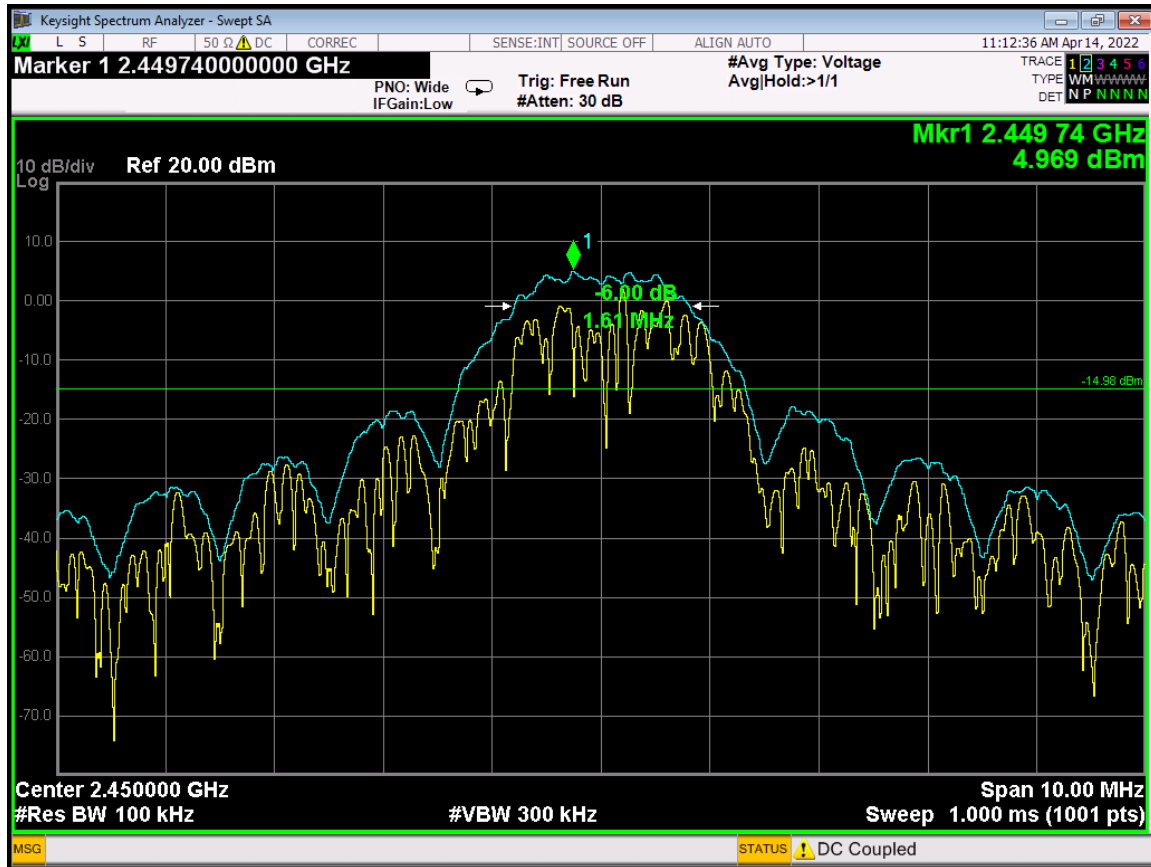
Bandwidth 6 dB - 2450 MHz
