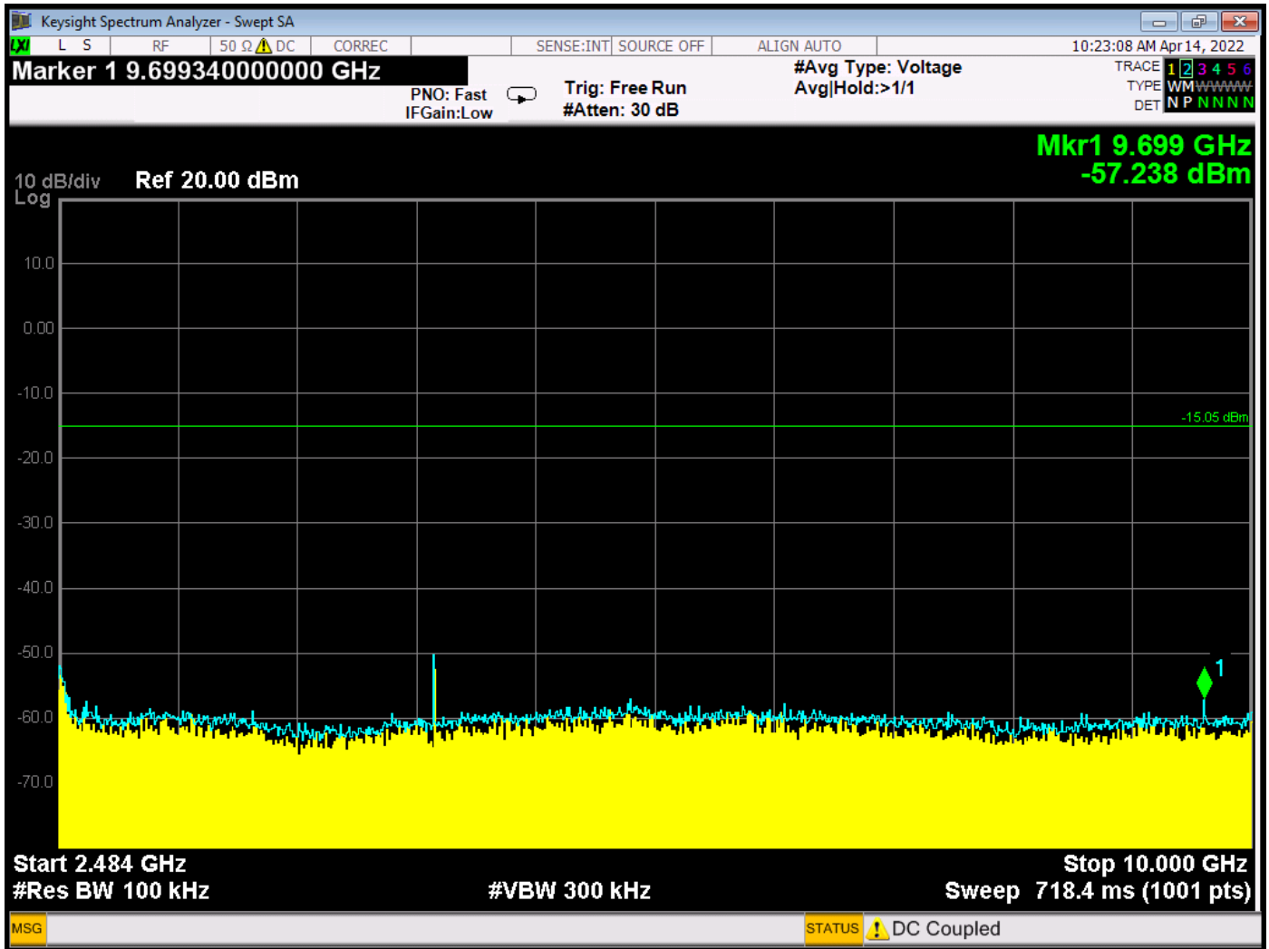
RF Antenna Conducted Test – Low Channel – 2483.5 MHz to 10 GHz
