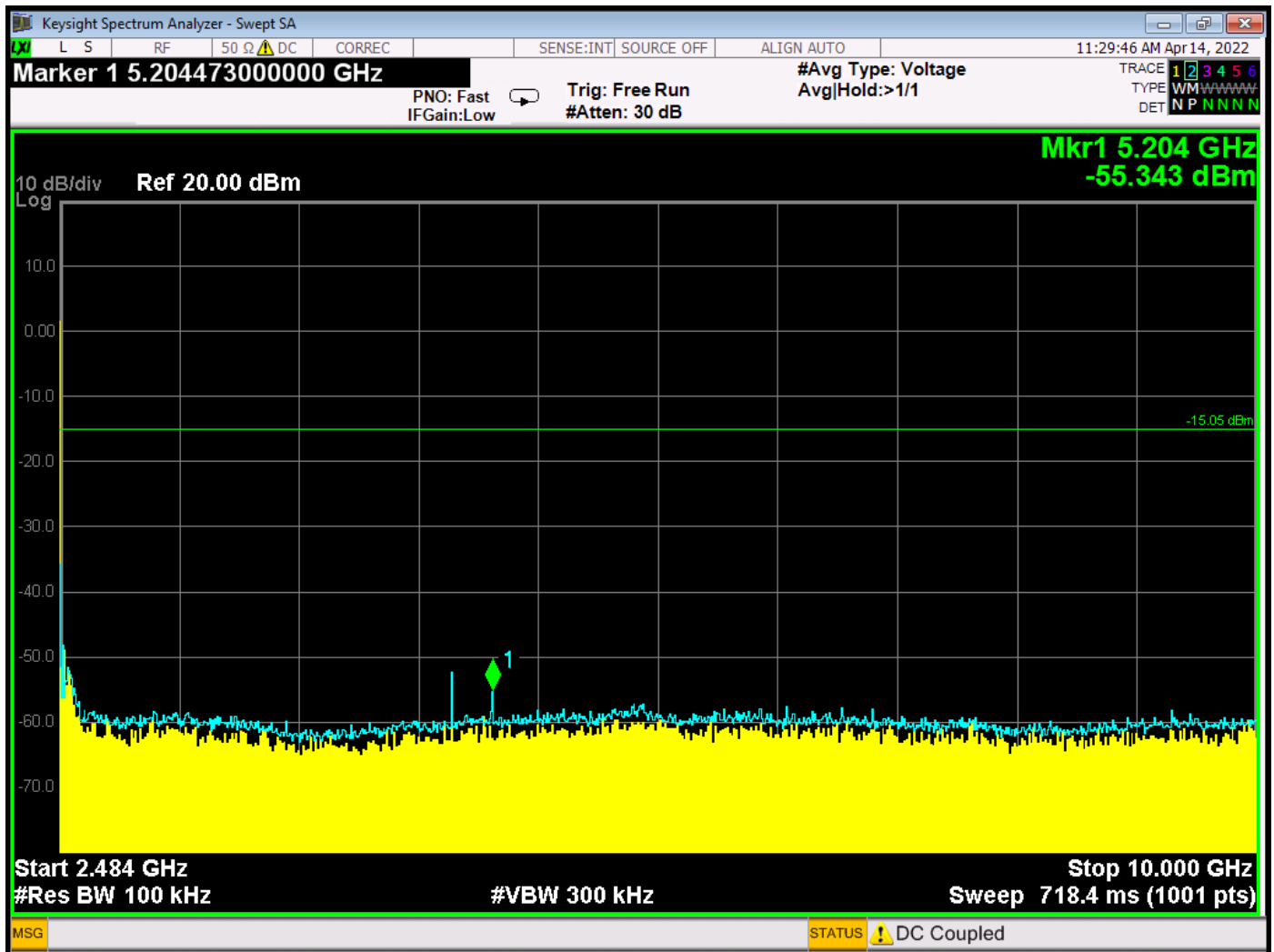
RF Antenna Conducted Test – High Channel – 2483.5 MHz to 10 GHz
