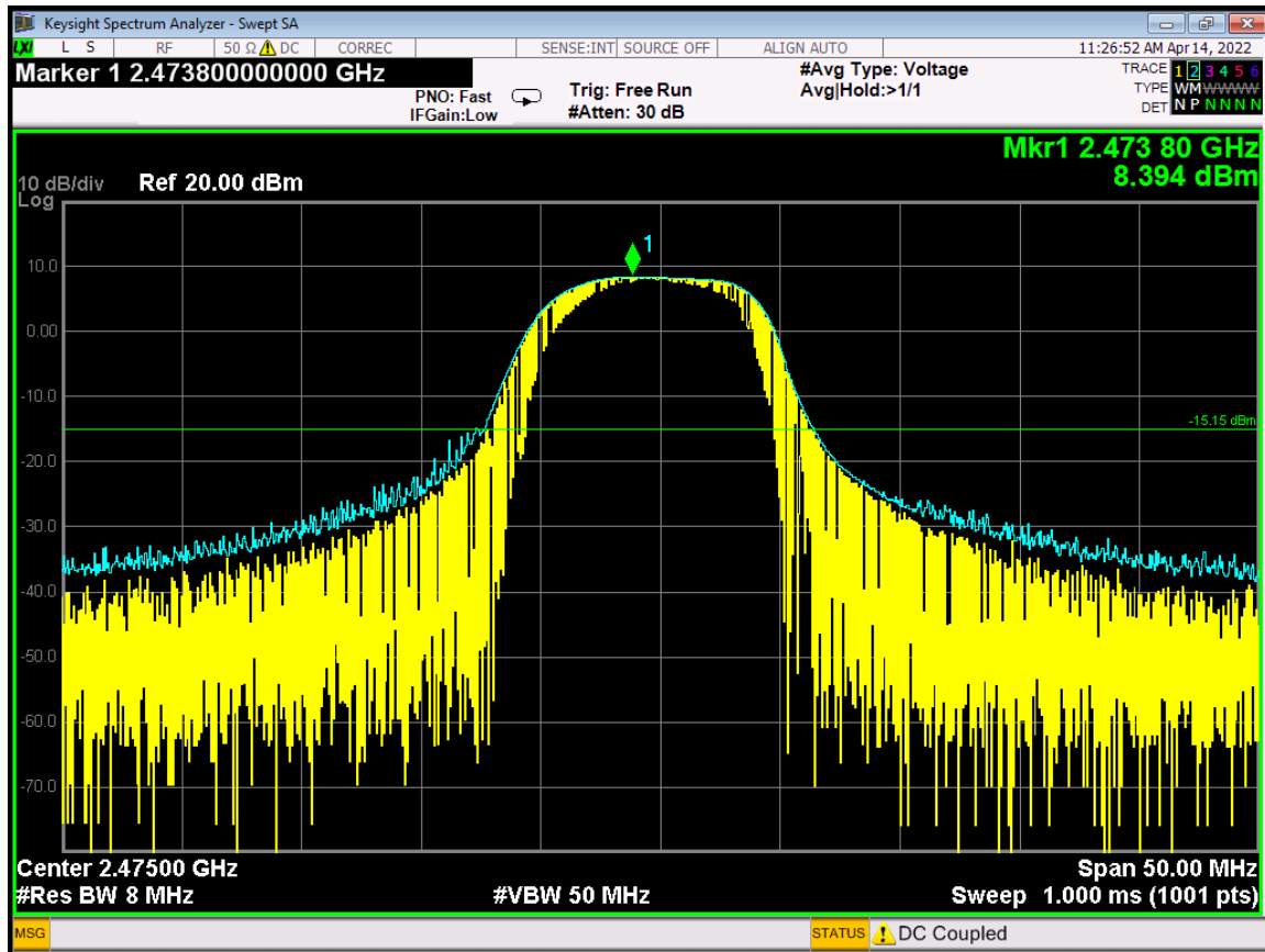
Peak Power Output - 2475 MHz
