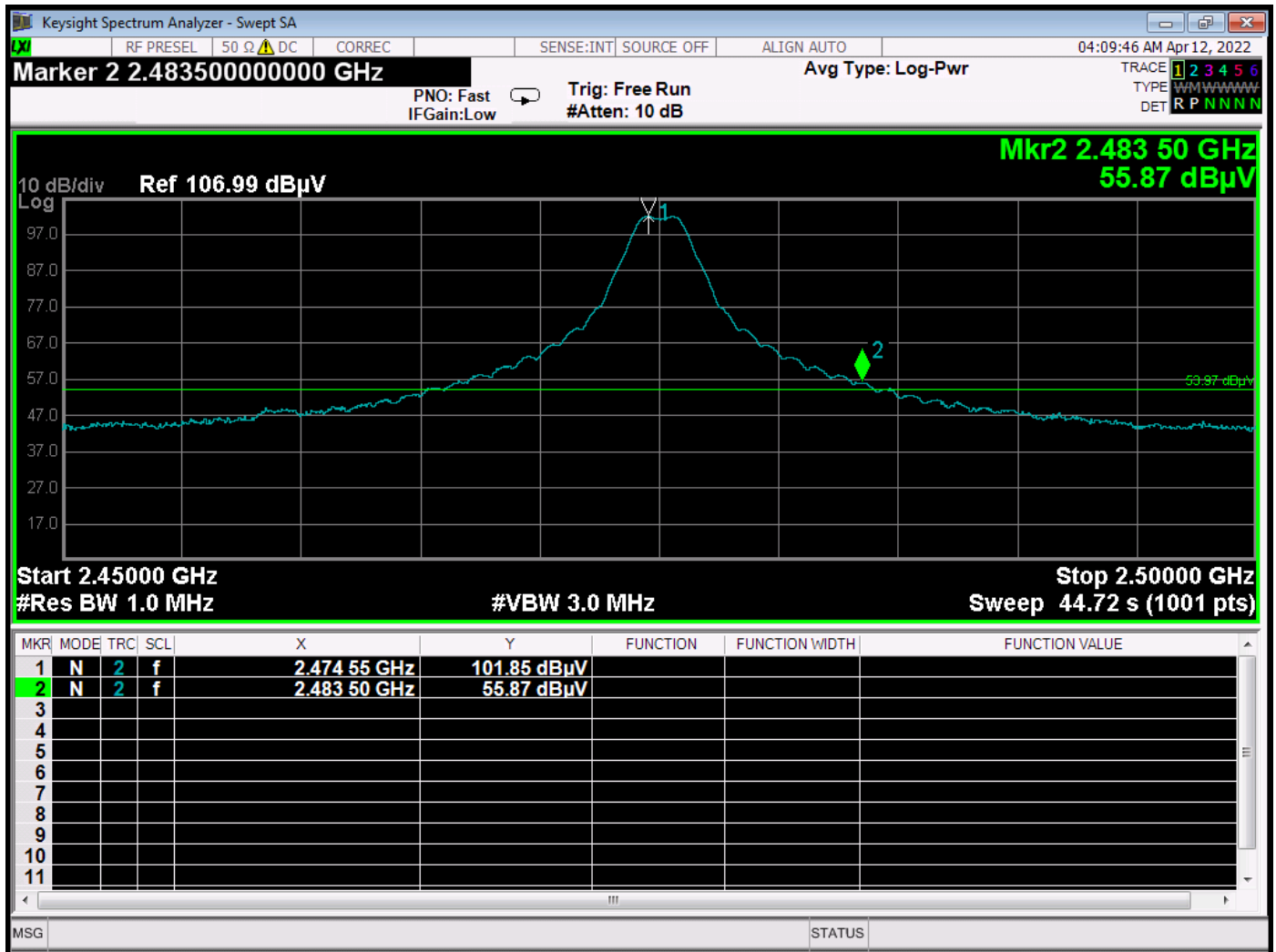
BE - 2475 MHz - Vertical - Z-Axis - Worst Case
