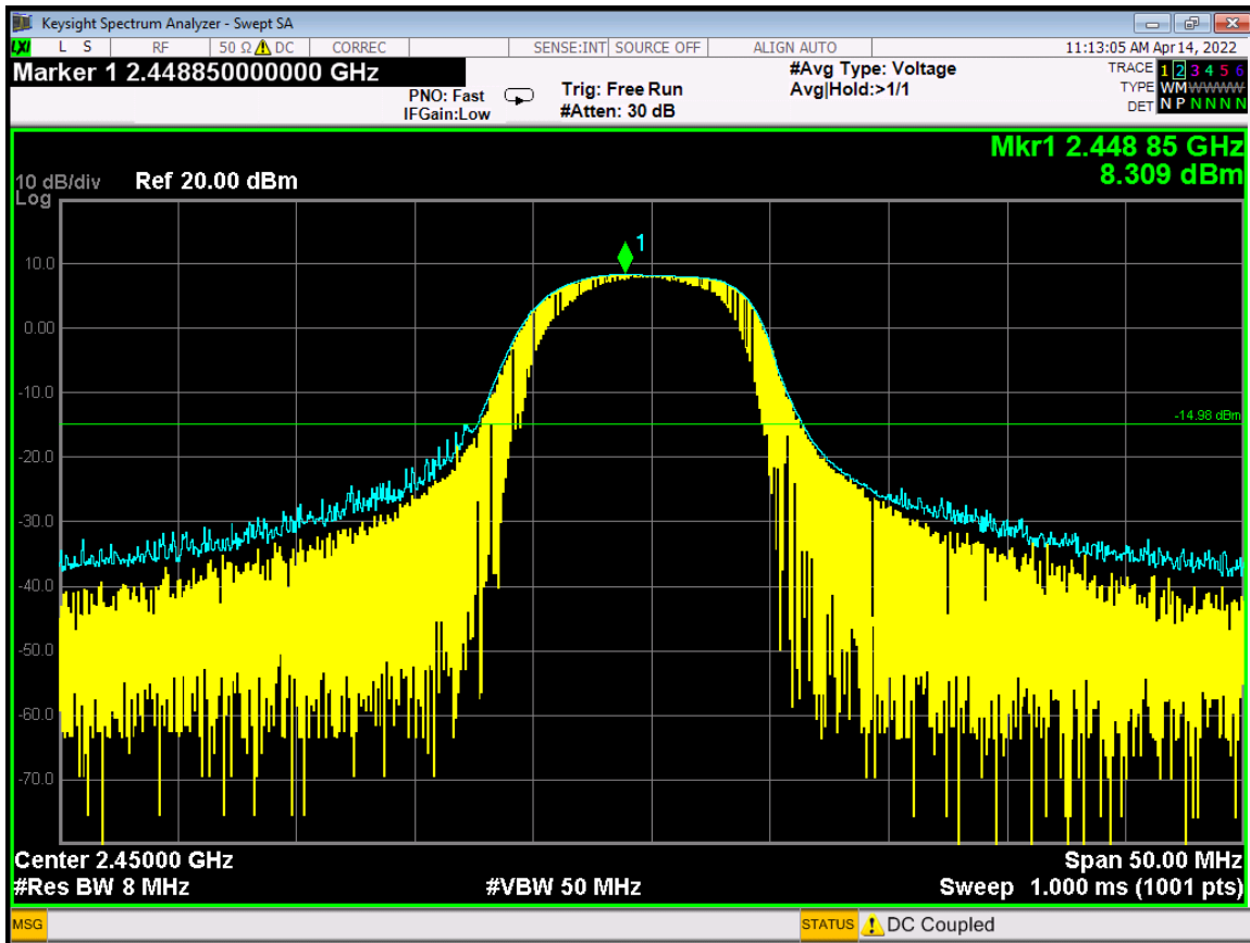
Peak Power Output - 2450 MHz
