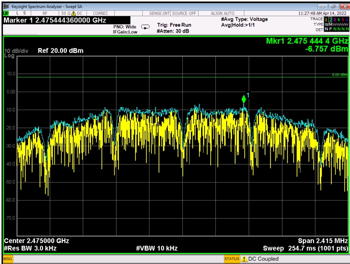
Special Density Output - 2475 MHz
