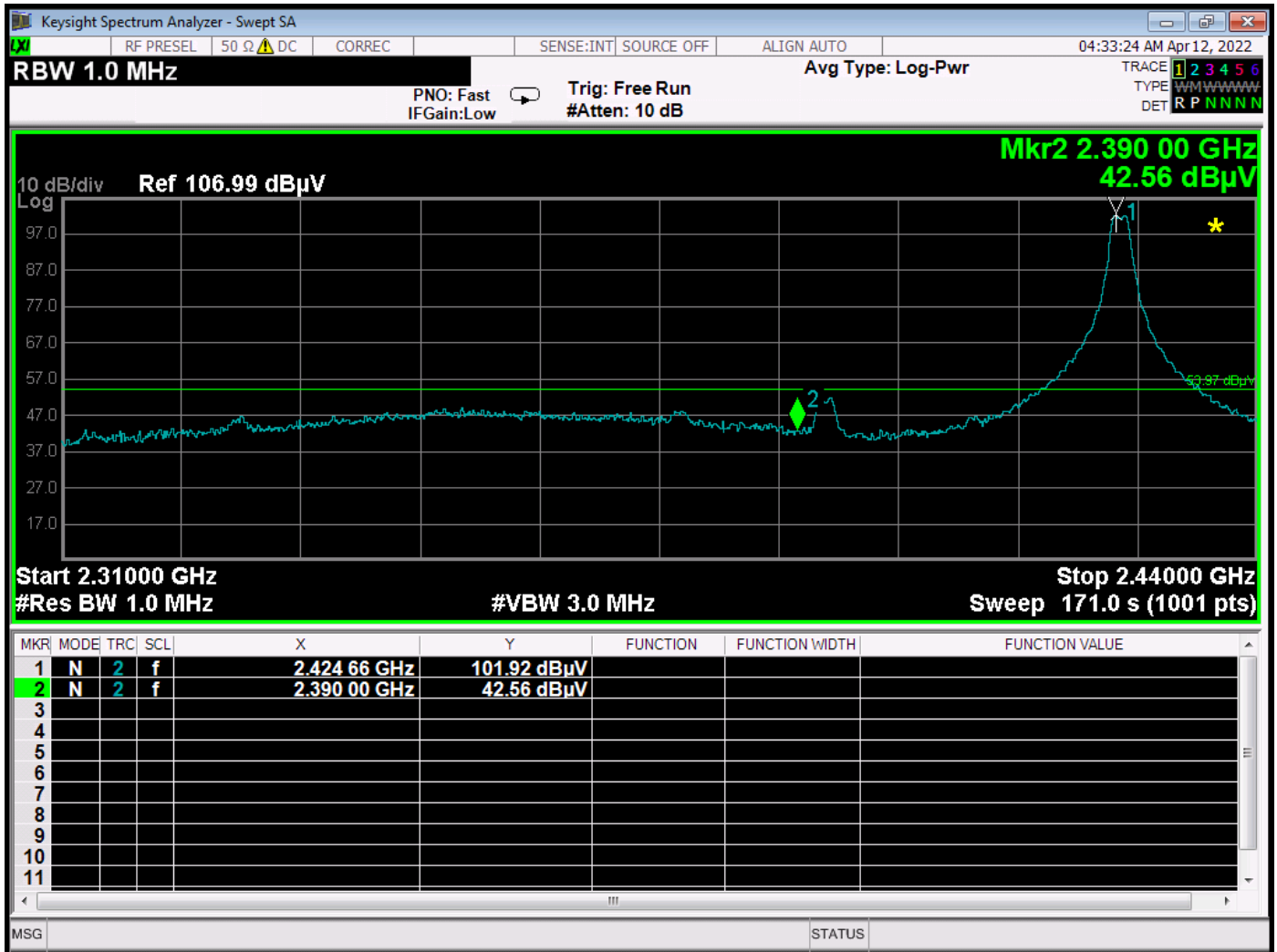
BE - 2425 MHz - Vertical - Z-Axis - Worst Case
