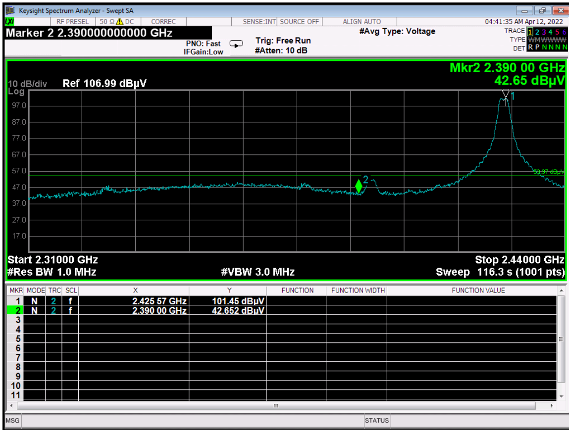
BE - 2425 MHz - Horizontal - X-Axis - Worst Case
