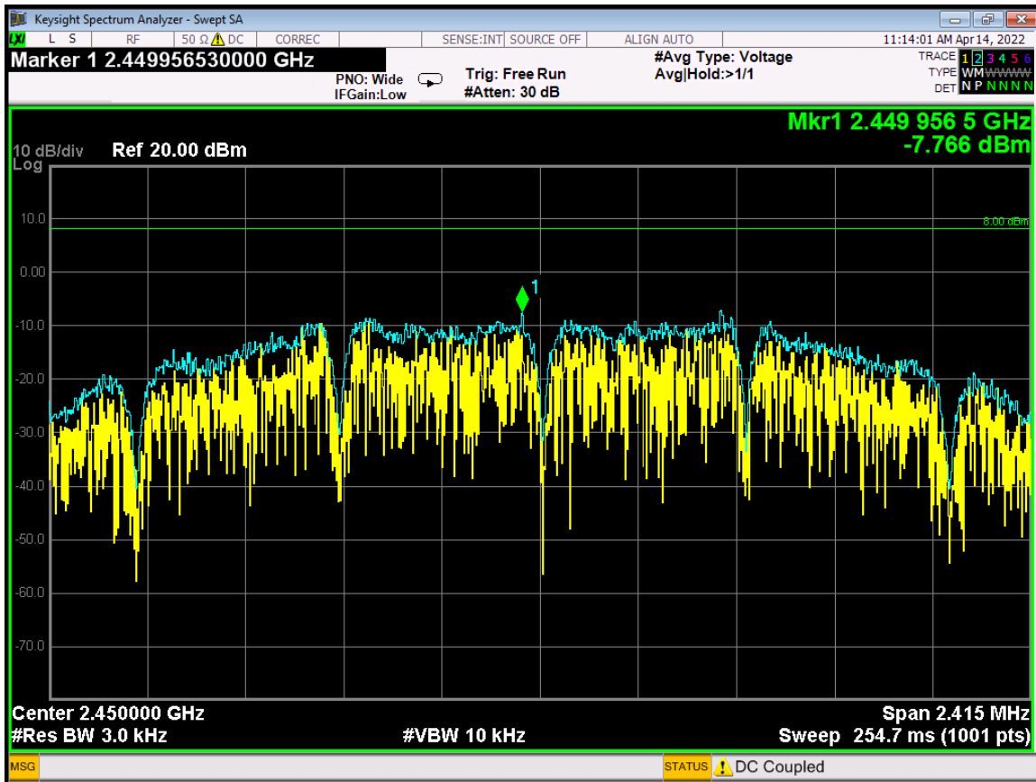
Special Density Output - 2450 MHz
