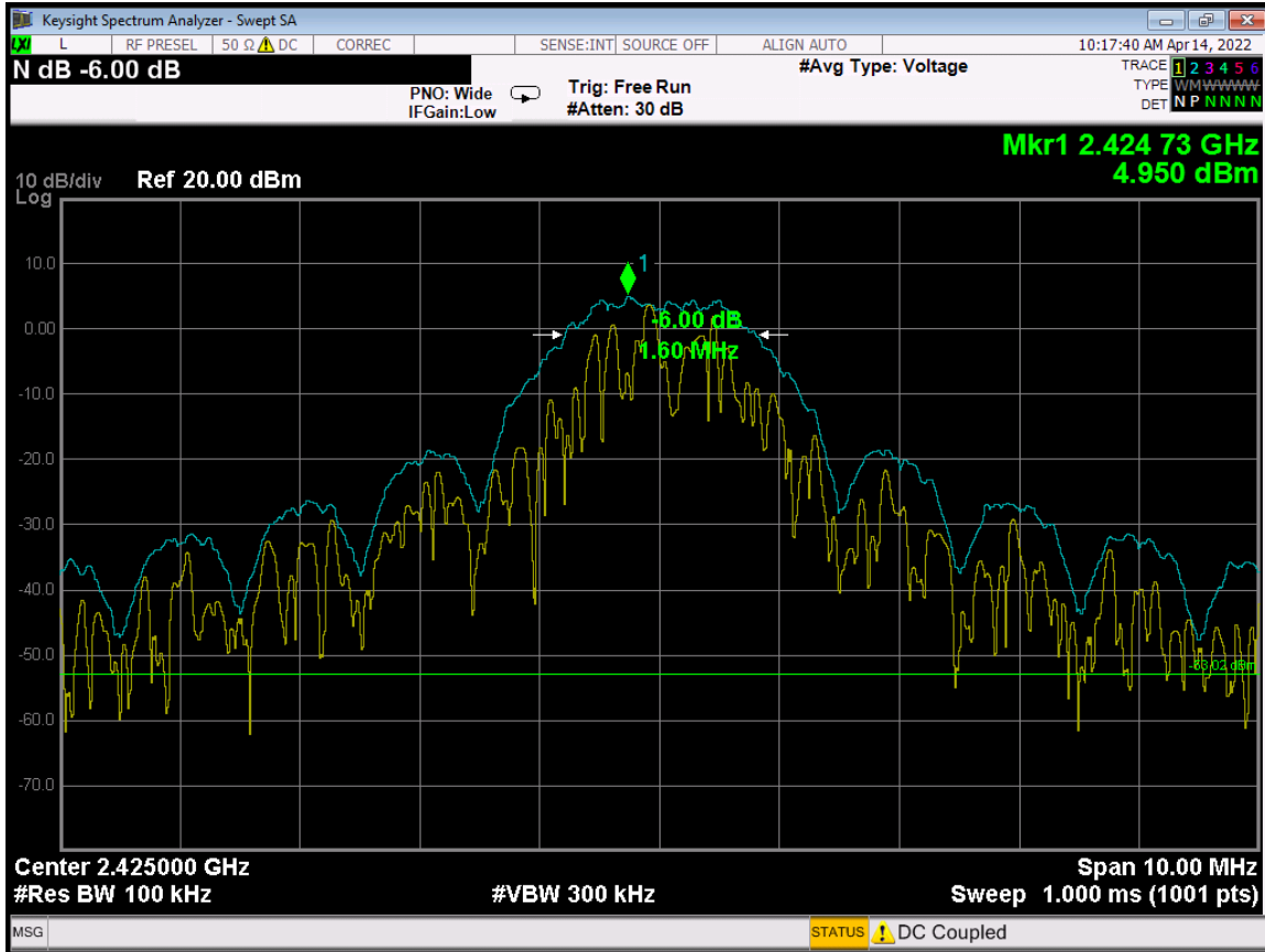
Bandwidth 6 dB - 2425 MHz
