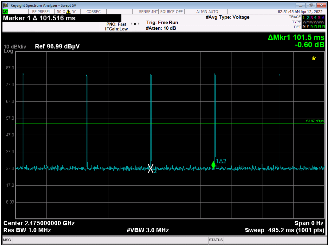
Time Between Pulses is 101.5 ms – Data Mode
