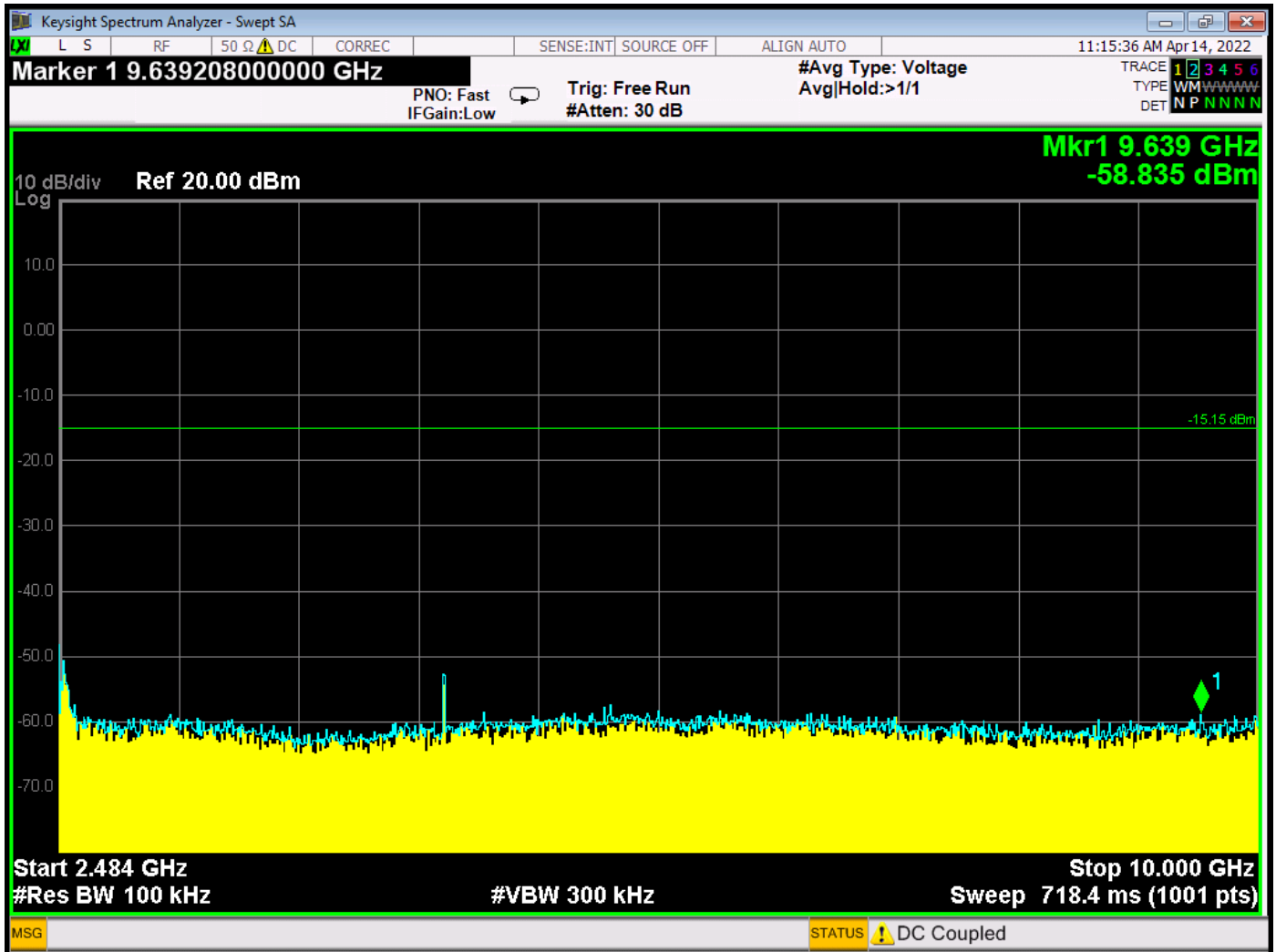
RF Antenna Conducted Test – Middle Channel – 2483.5 MHz to 10 GHz
