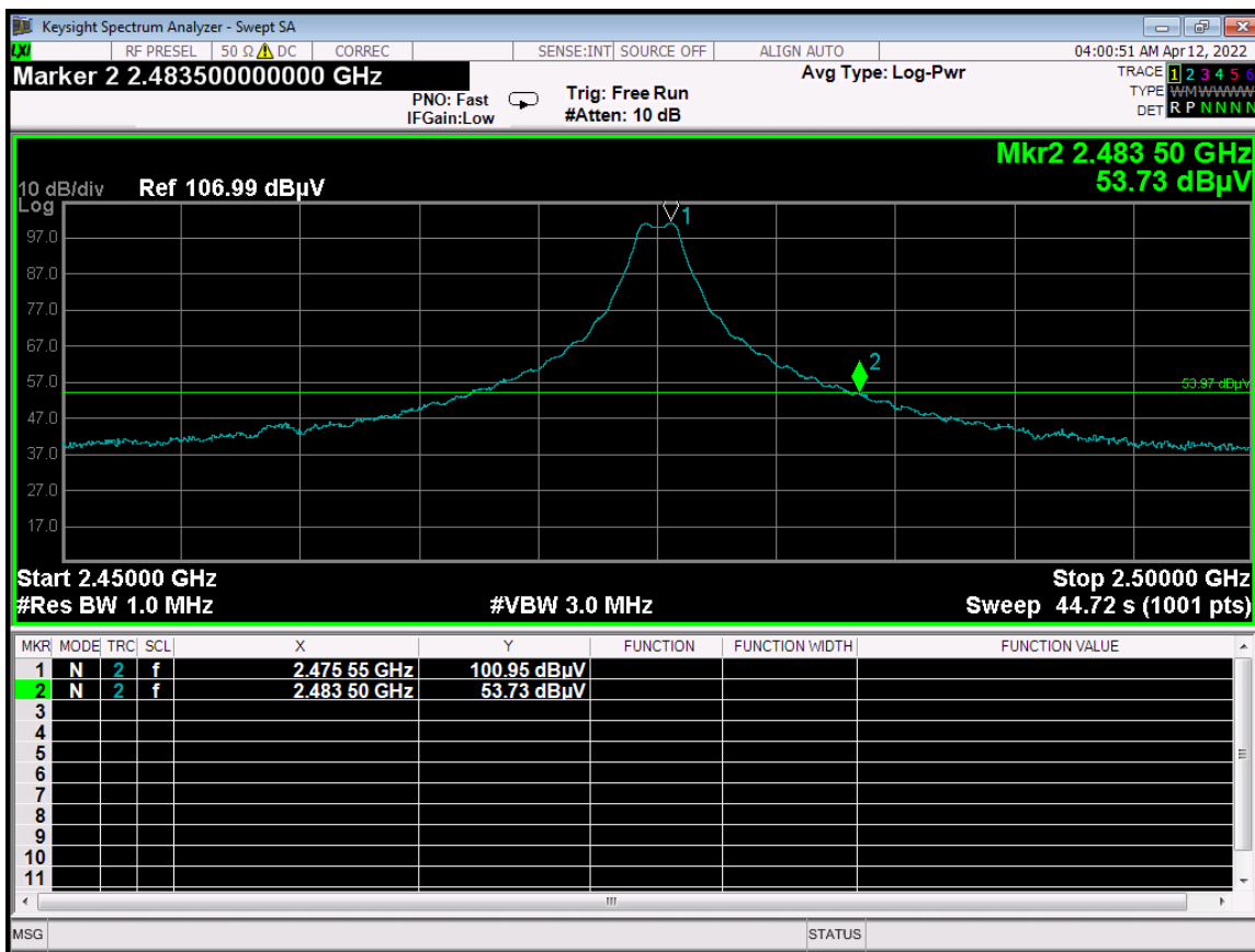
BE - 2475 MHz - Horizontal - X-Axis - Worst Case
