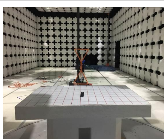
Radiated Emissions (<1GHz) – Rear View
