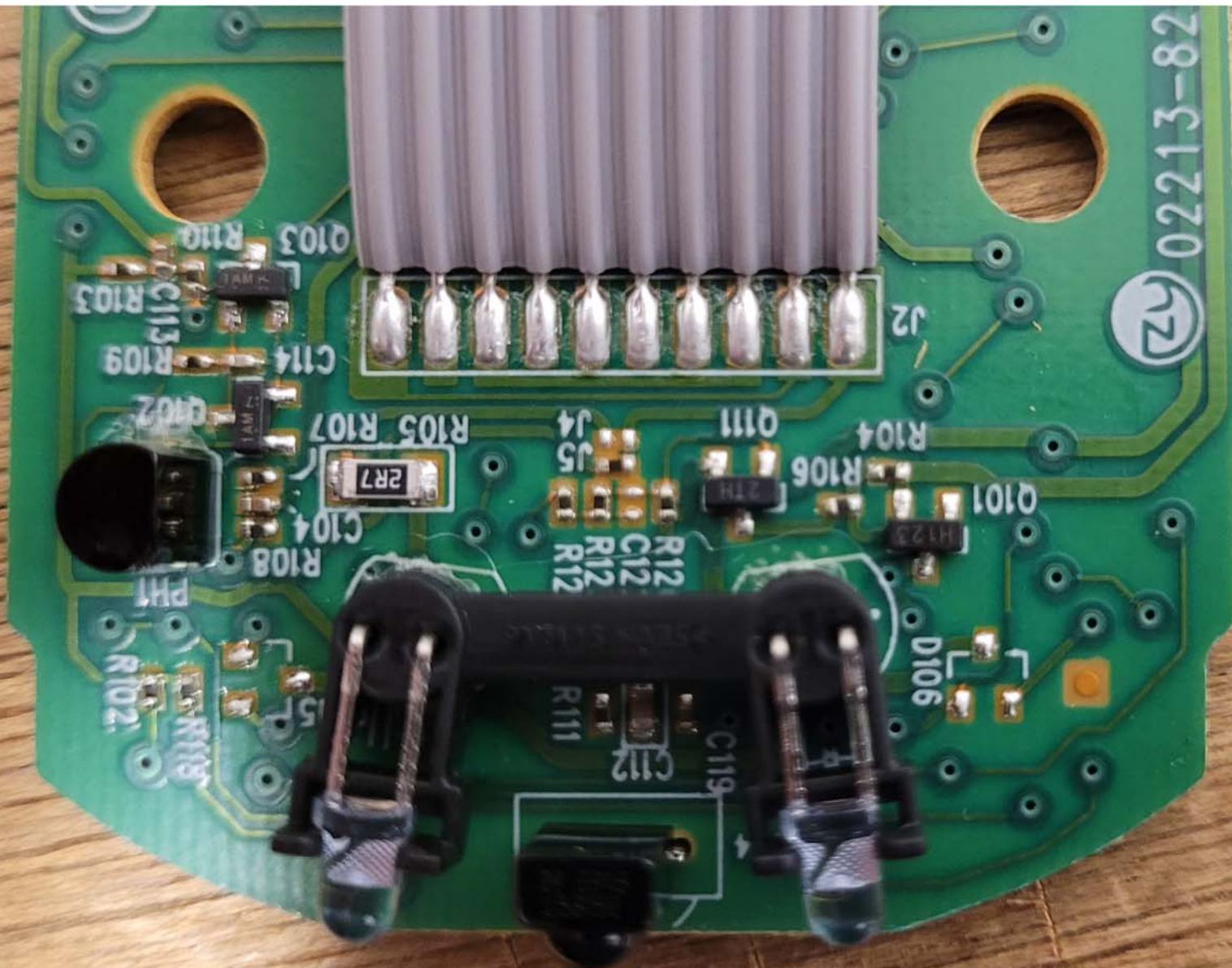
Bottom View of the PCB - Closeup #8
