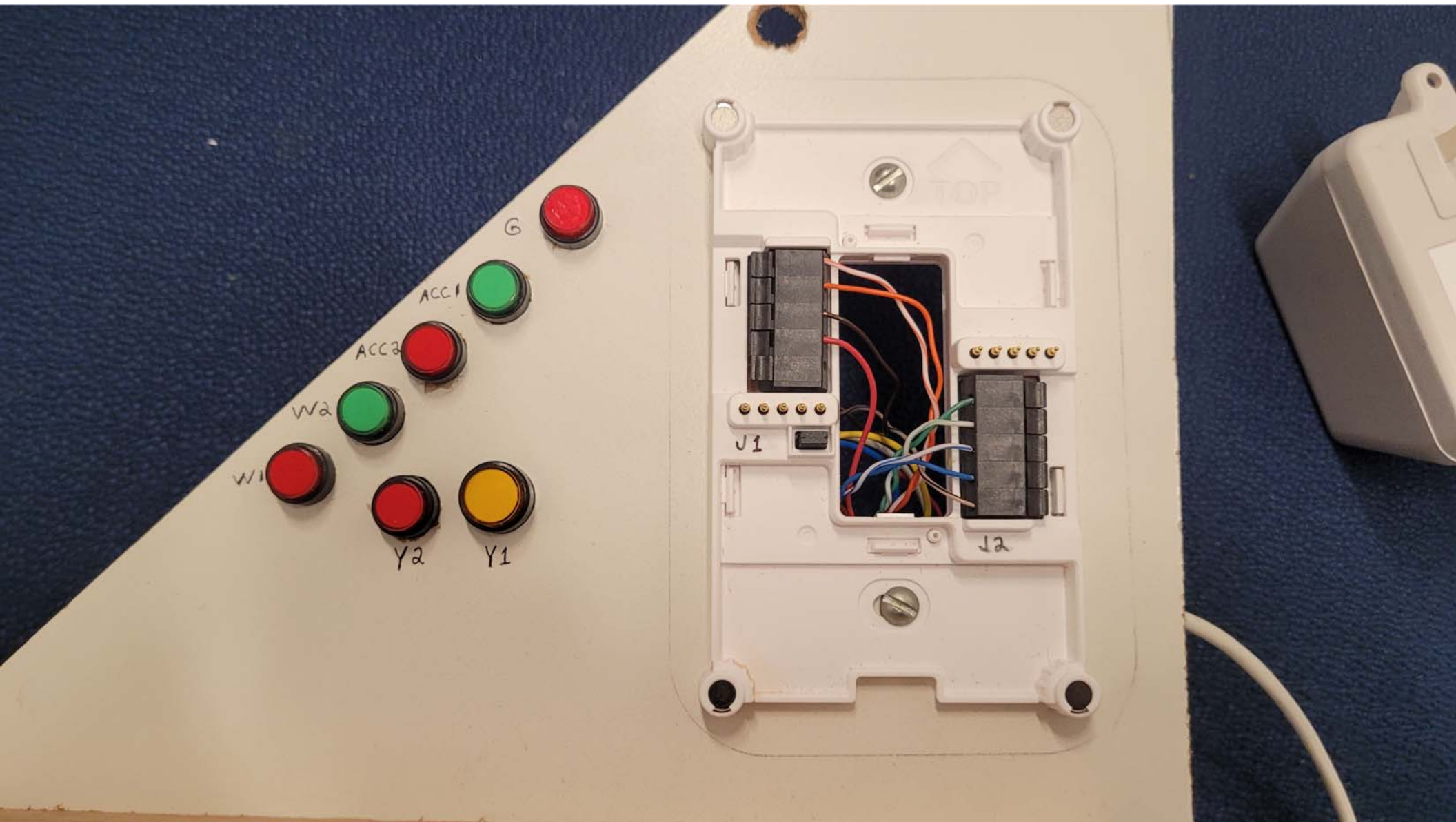
Mounting Device - Front View
