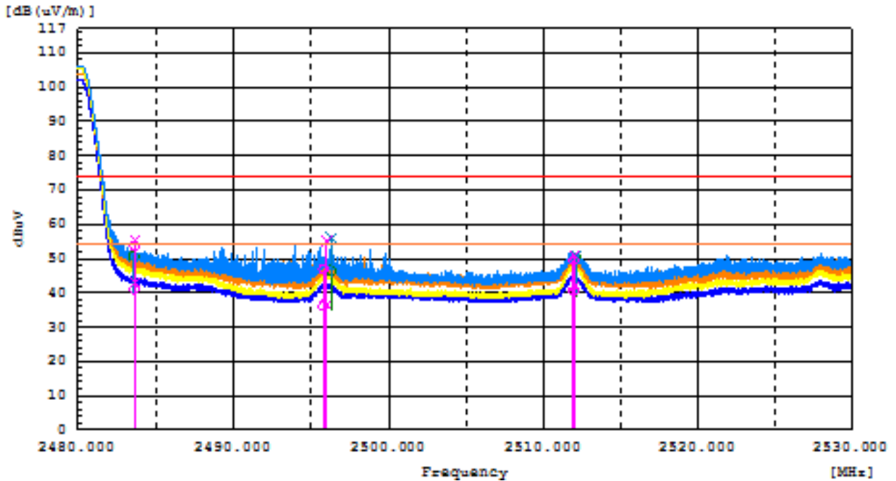
Radiated Restricted Band Edges plot – ANT1 (Ch.39)
