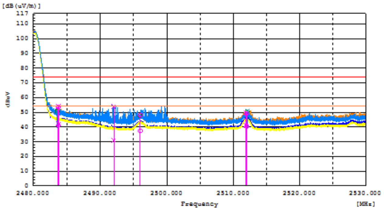
Radiated Restricted Band Edges plot – ANT1 (Ch.39)
