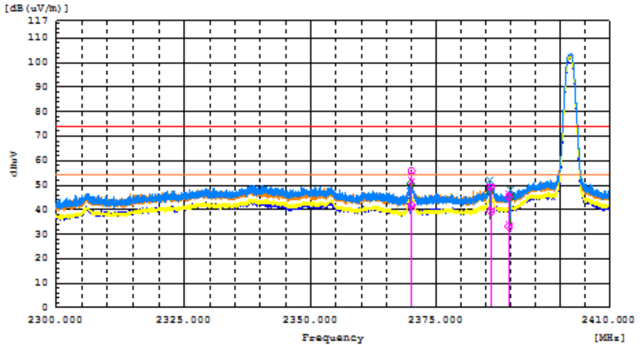
Radiated Restricted Band Edges plot – ANT0 (Ch.0)
