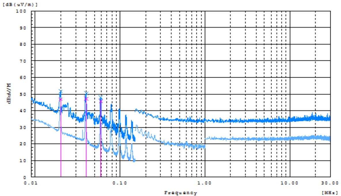
Radiated Spurious Emissions plot – ANT1 (Ch.39)
