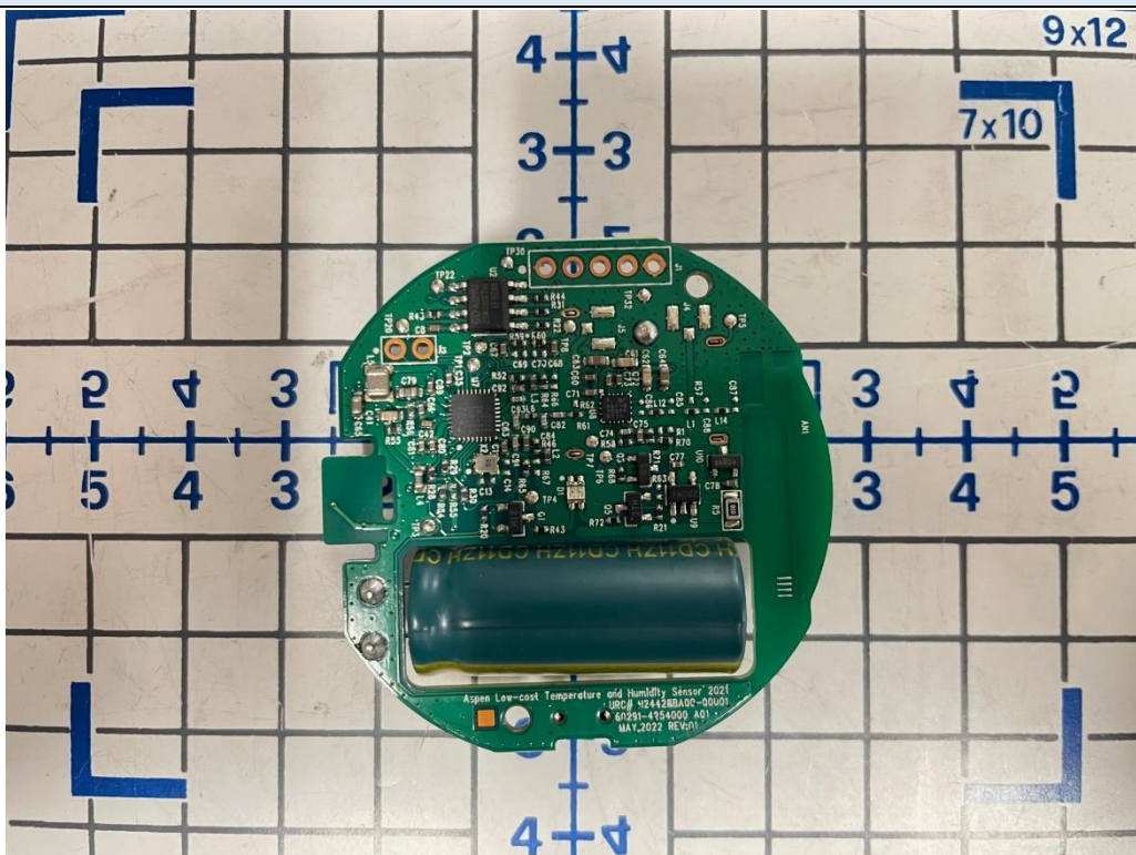
Mainboard View 2
