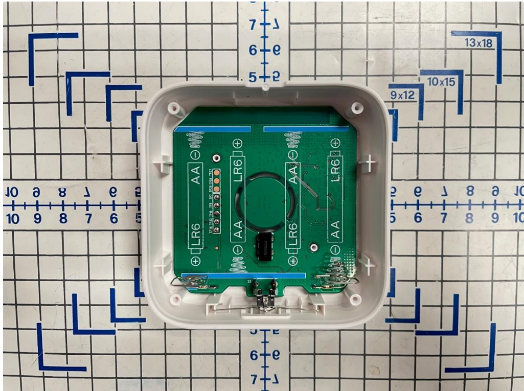
Mainboard View 2
