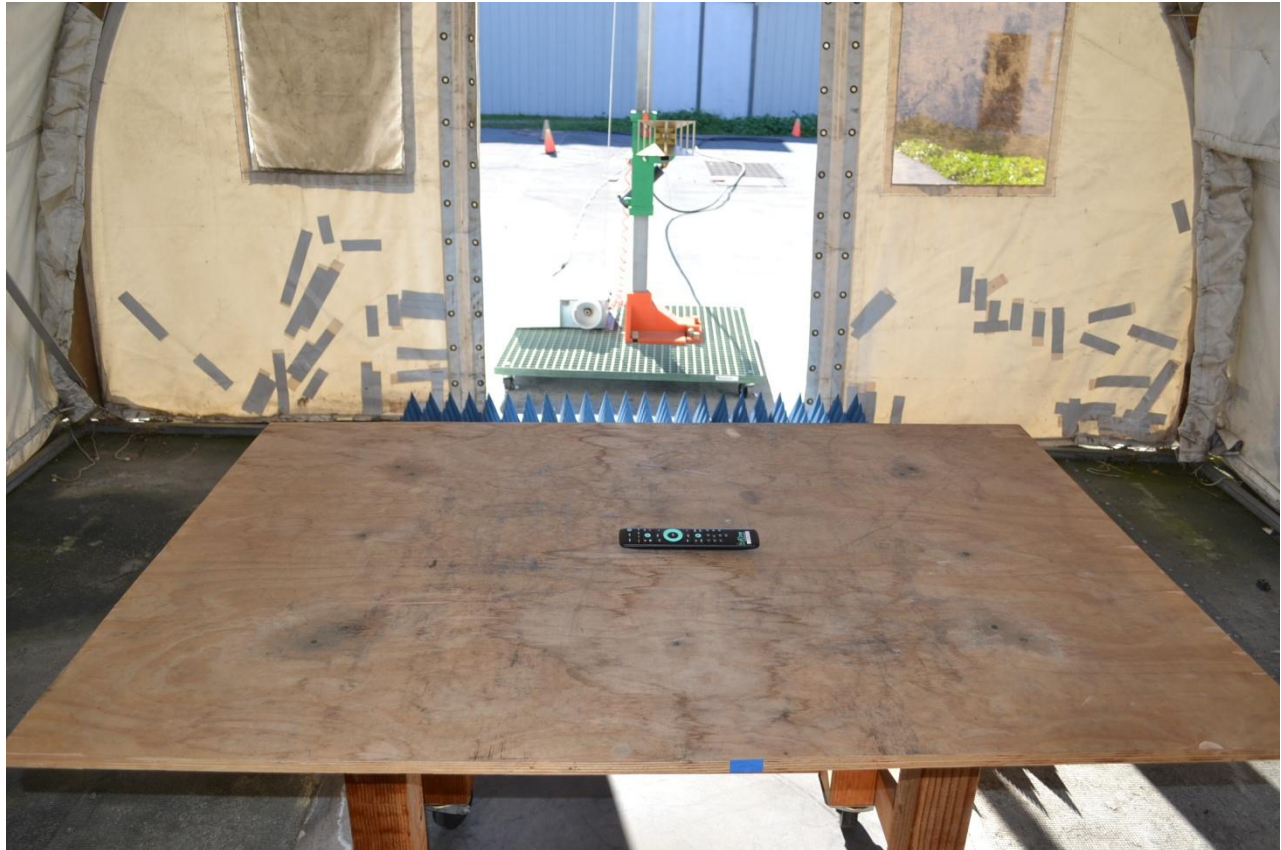
Radiated Emissions - 3 Meter Setup (>1 GHz)
