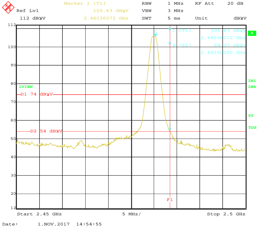
Band Edge - 2480 MHz - Horizontal - X-Axis - Worst Case
