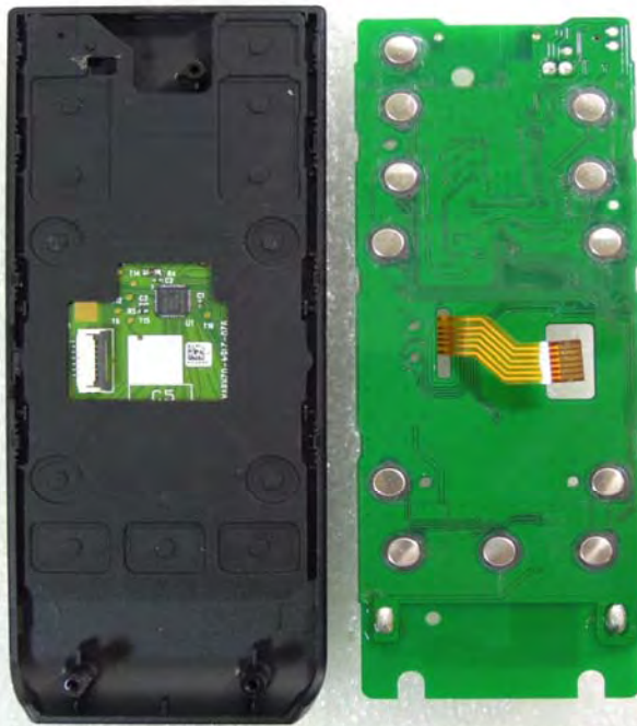
Open View of EUT – 4
