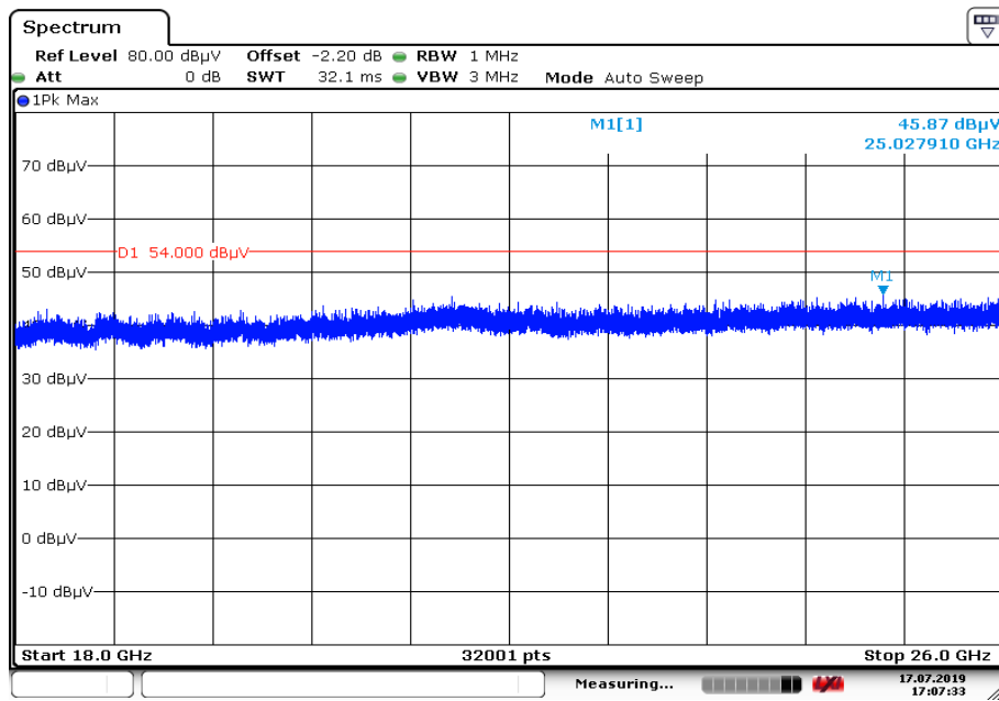
Plot 12: 18 GHz to 26 GHz, TX mode, 2480 MHz, vertical & horizontal polarization, Antenna 2
