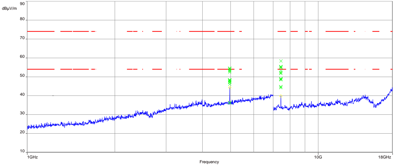
Plot 5: 1 GHz to 18 GHz, TX mode, 2480 MHz, vertical & horizontal polarization, Antenna 1
