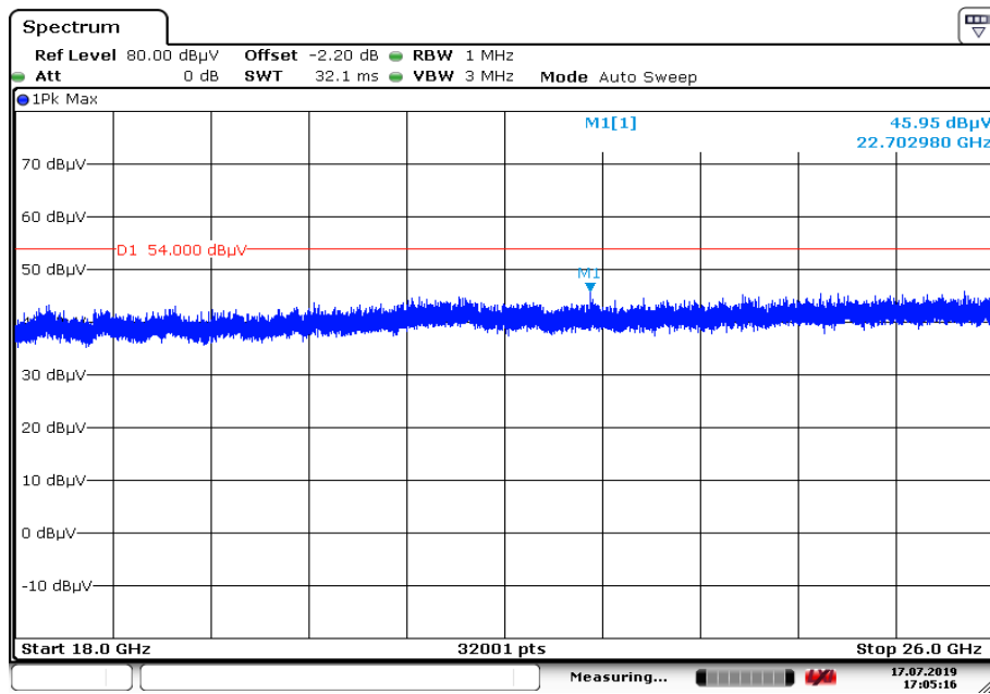
Plot 4: 18 GHz to 26 GHz, TX mode, 2440 MHz, vertical & horizontal polarization, Antenna 1
