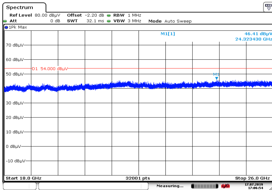
Plot 8: 18 GHz to 26 GHz, TX mode, 2405 MHz, vertical & horizontal polarization, Antenna 2
