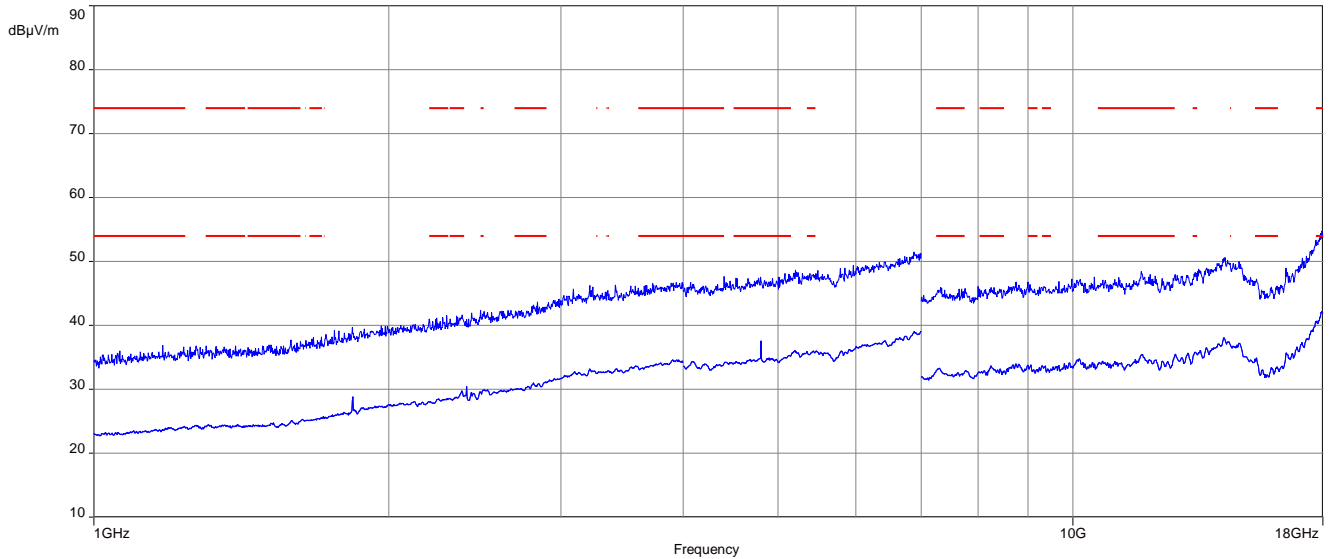
Plot 1: 1 GHz to 18 GHz, TX mode, 2402 MHz, vertical & horizontal polarization, 1 Msp
