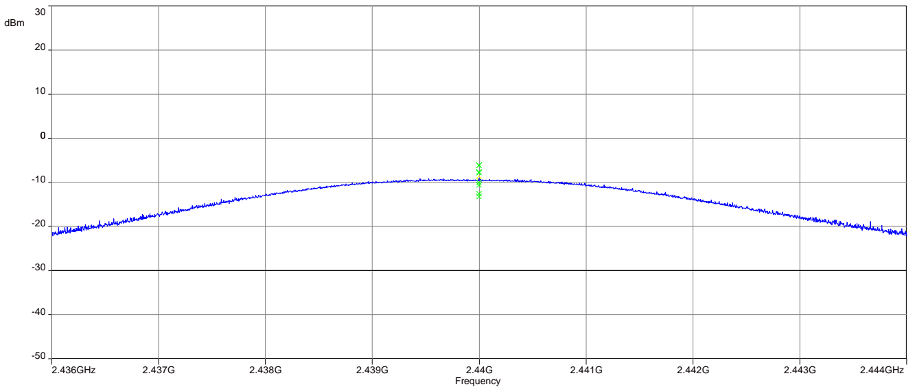
Plot 2: Mid channel, 1 Msps
