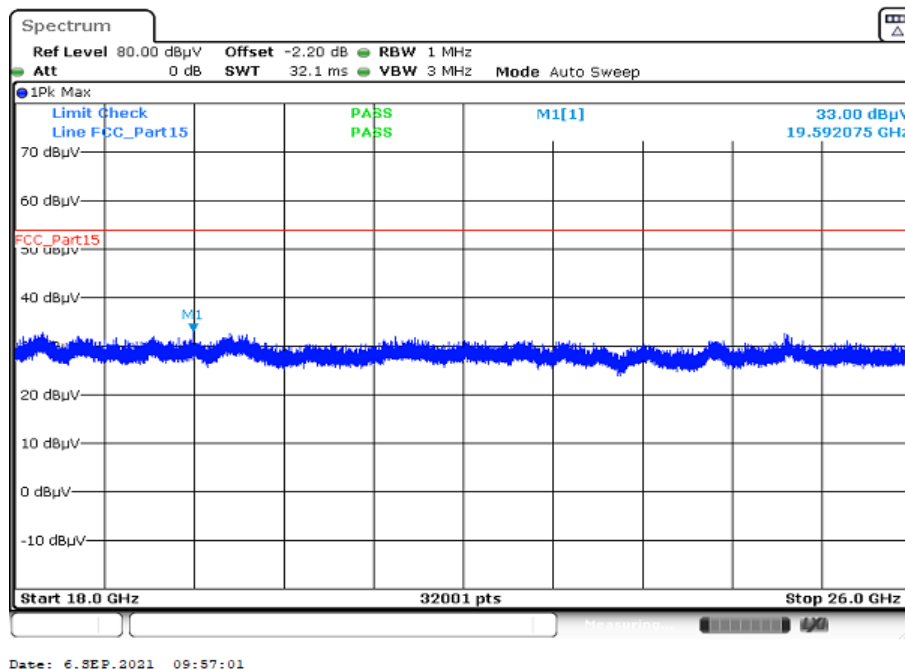
Plot 2: 18 GHz to 26 GHz, TX mode, 2402 MHz, vertical & horizontal polarization, 1 Msp
