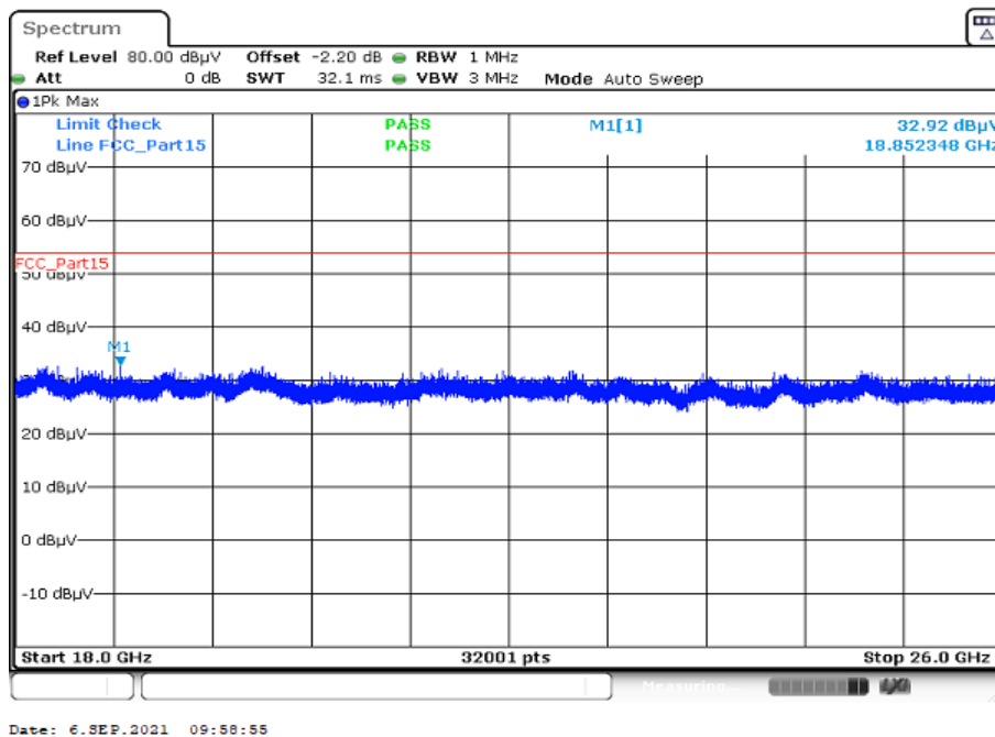
Plot 6: 18 GHz to 26 GHz, TX mode, 2480 MHz, vertical & horizontal polarization, 1 Msp
