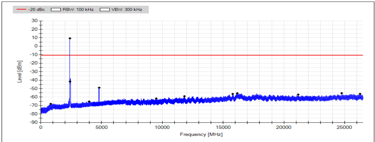
Figure 38: Conducted spurious emissions 30 - 26500 MHz channel 0, power setting 145, PHY 125k
