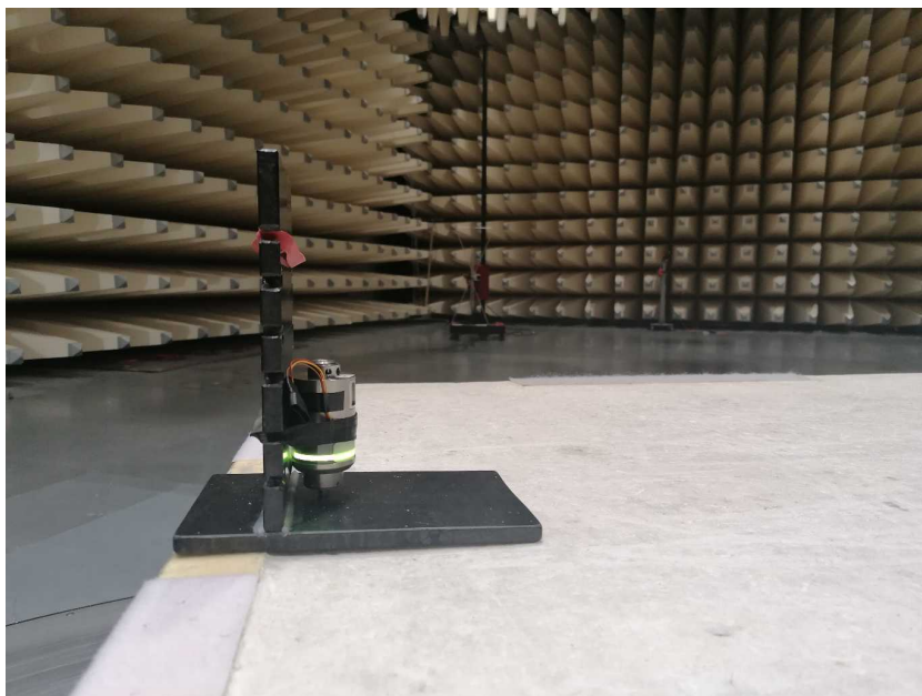
Photo 8 RSE 30-1000MHz
