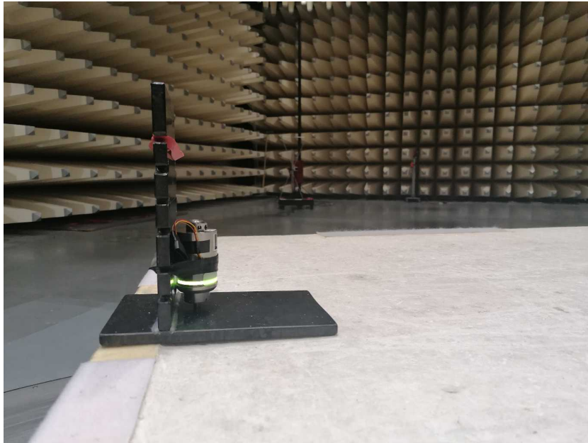
Photo 9 RSE 30-1000MHz
