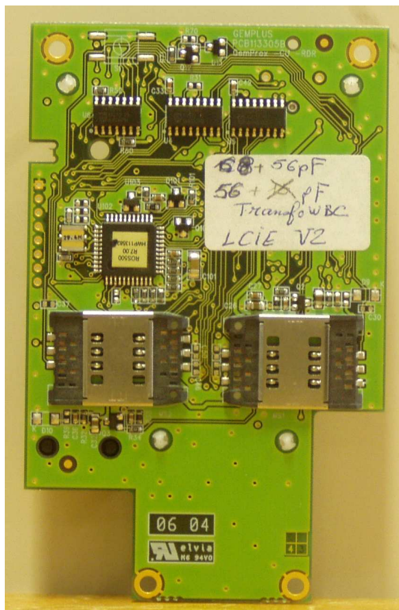
RF board
