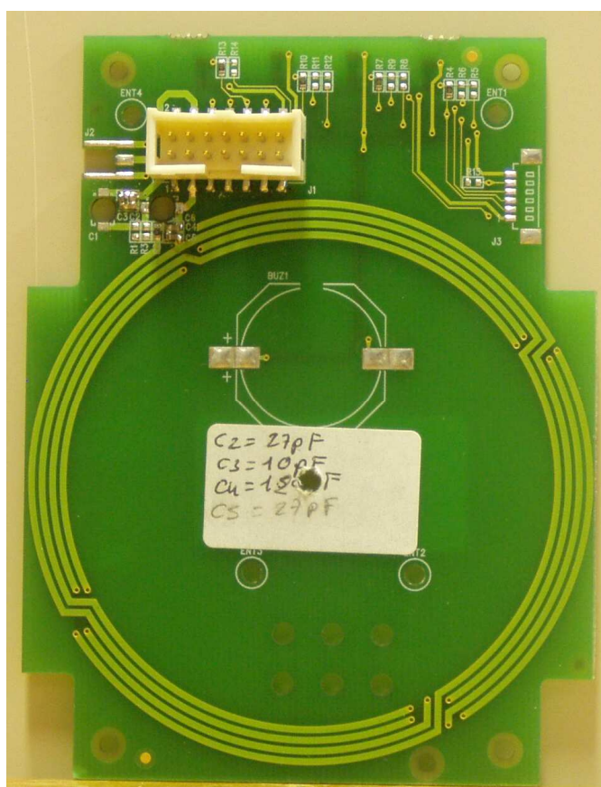
Antenna board
