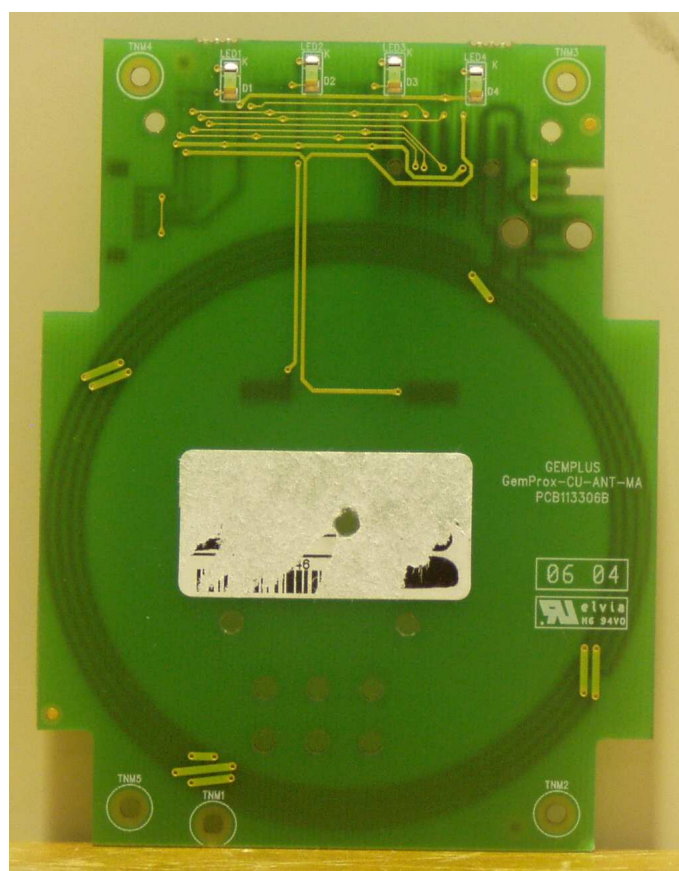
Antenna board
