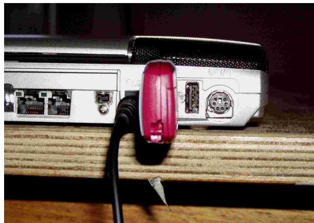
Detail view (EUT directly plugged into the USB port of the PC)
